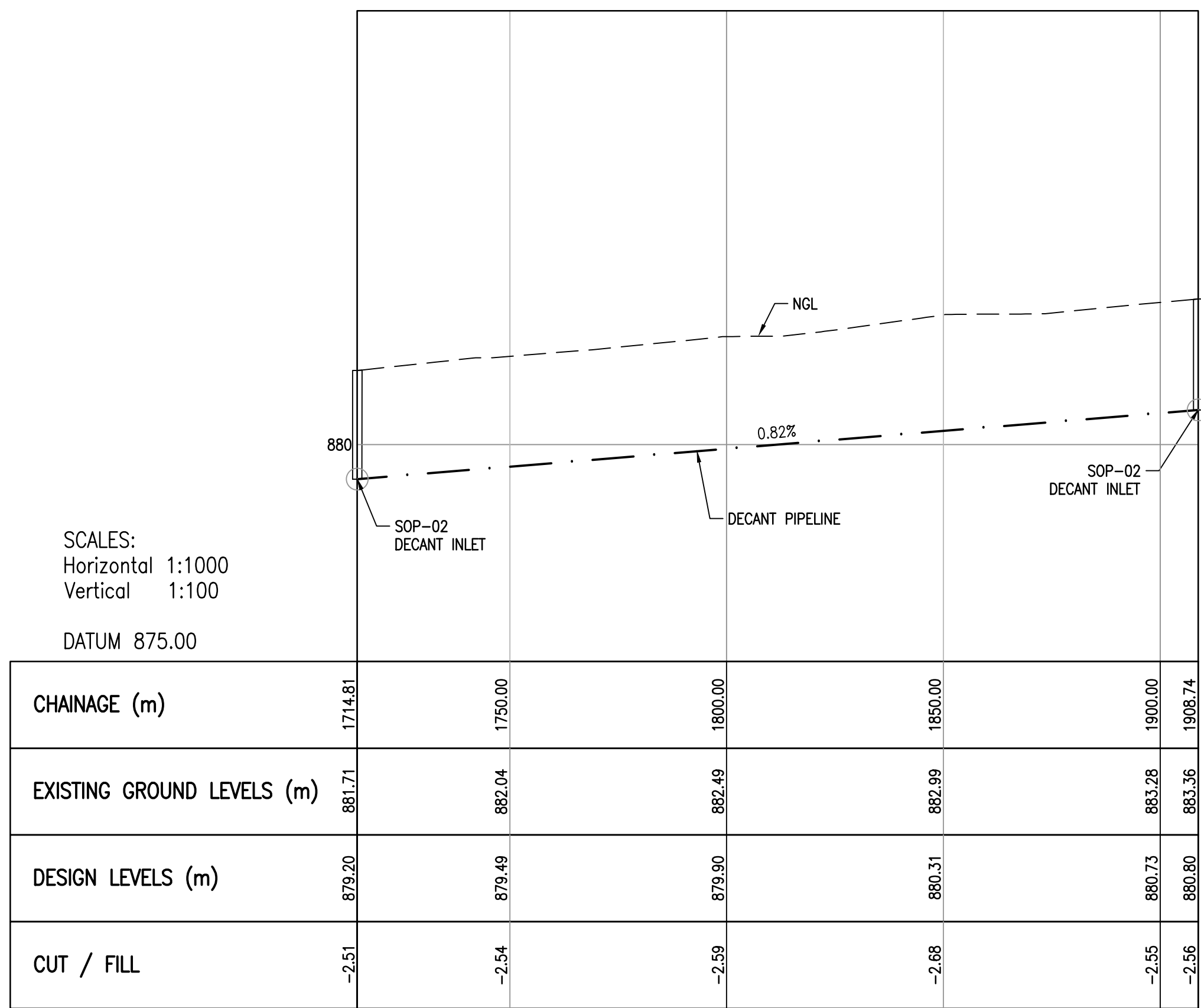
CLEAN WATER DECANT PIPELINE LONGITUDINAL SECTION CH. 1714.82 TO CH. 1908.74 SCALE 1:1000
