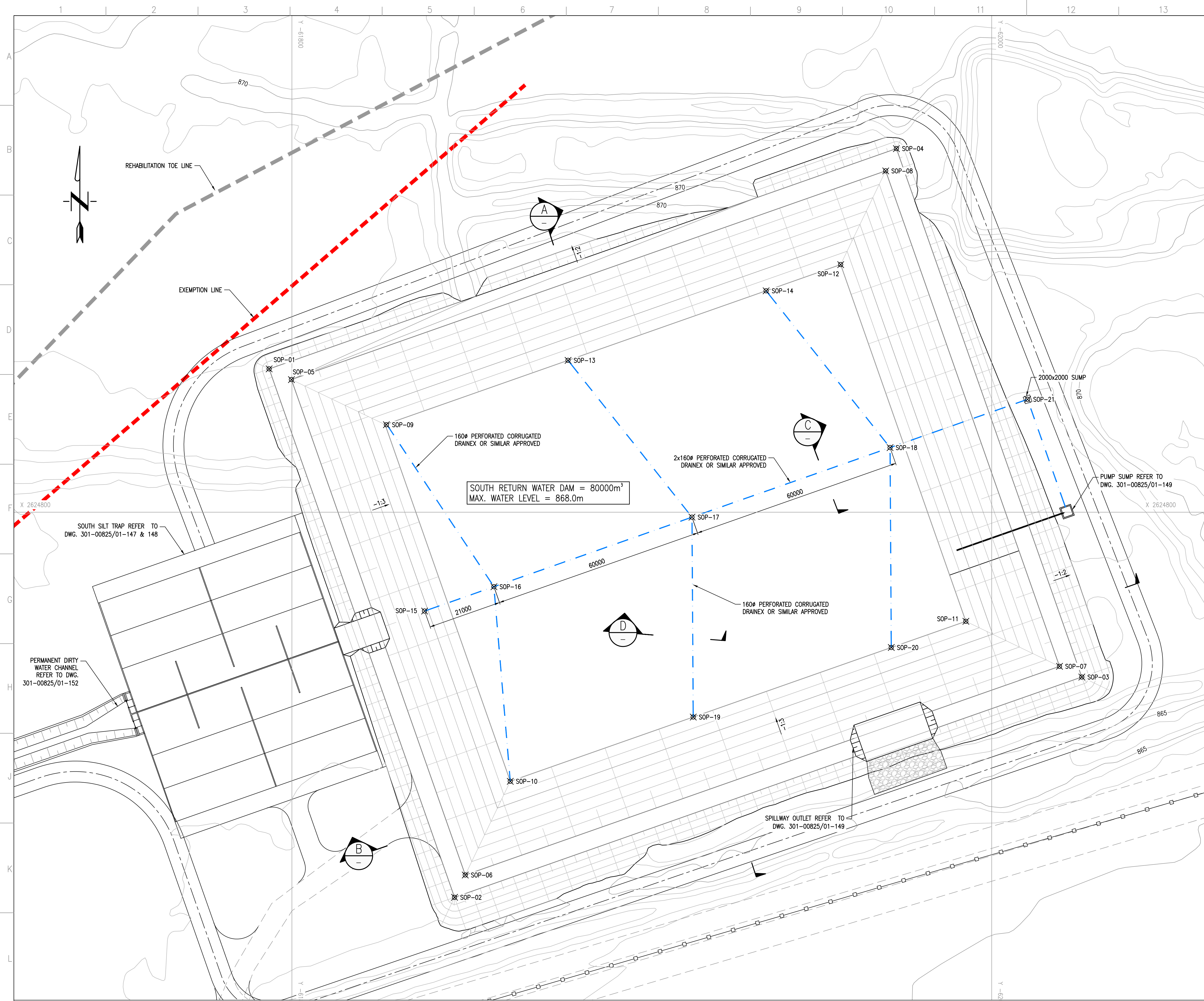
SOUTH RETURN WATER DAM LAYOUT PLAN SCALE 1:500
