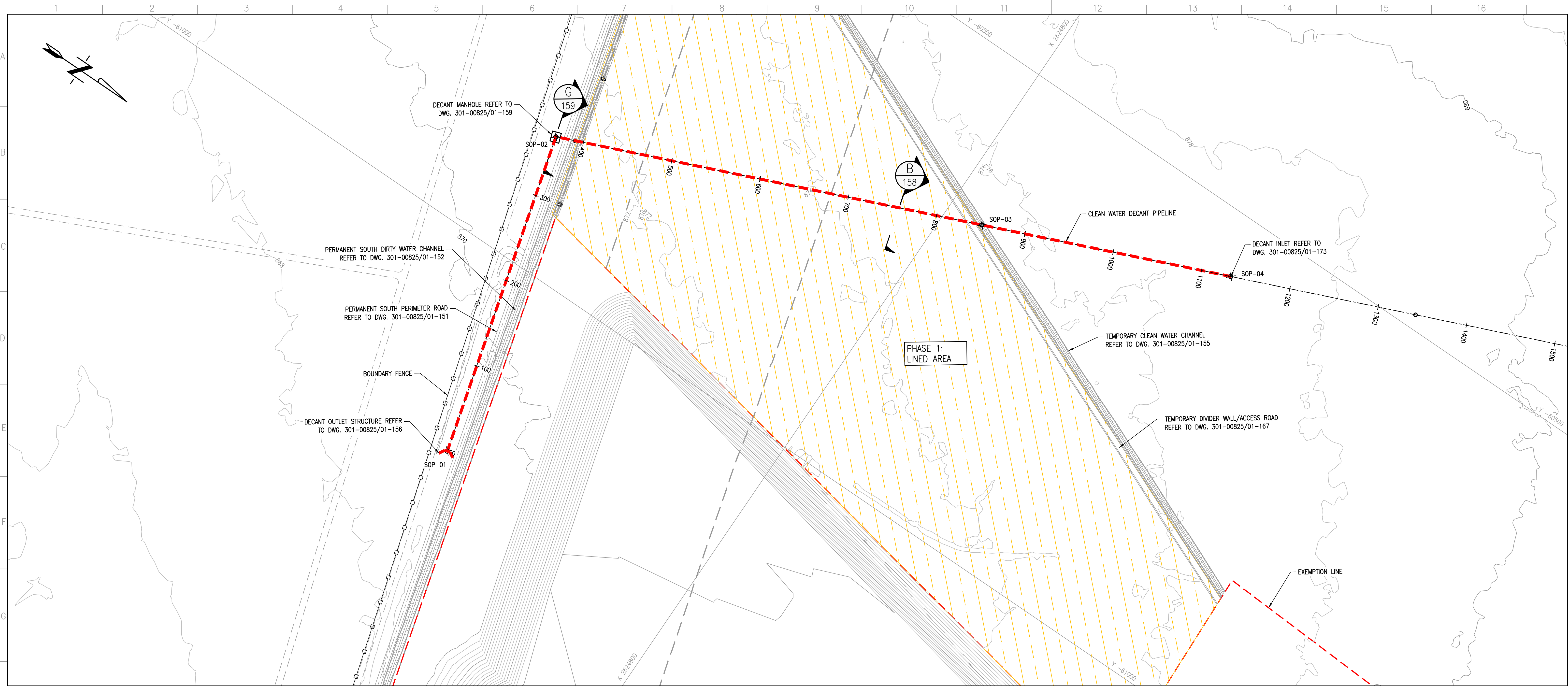
CLEAN WATER DECANT PIPELINE LAYOUT PLAN SCALE 1:2000
