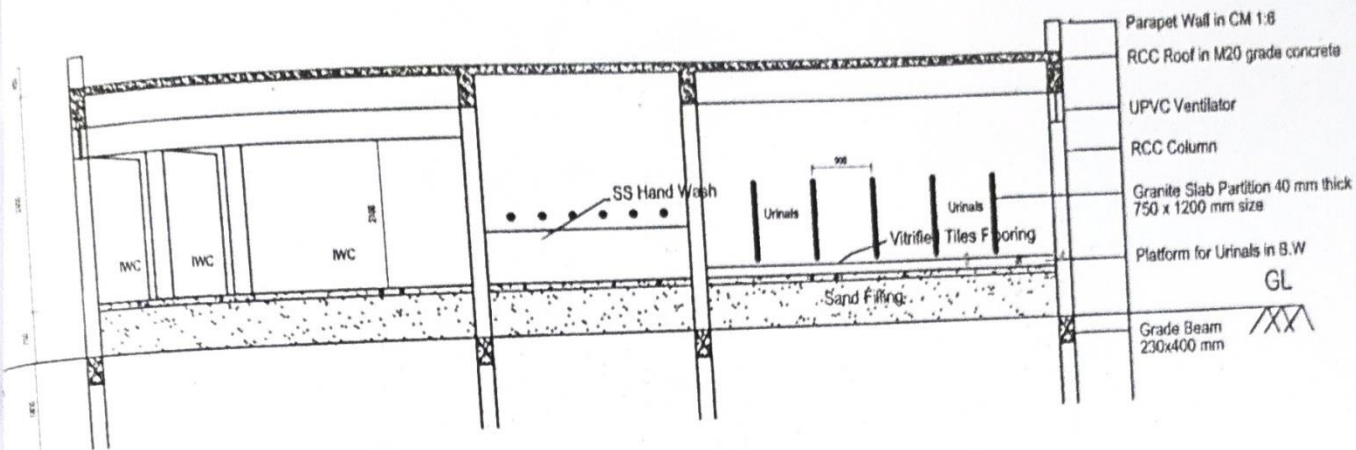
CROSS SECTION
