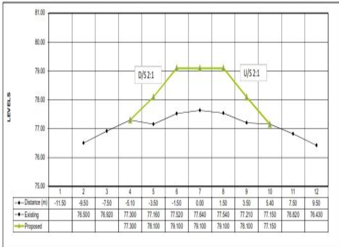
TYPICAL CROSS SECTION FOR TANK BUND
