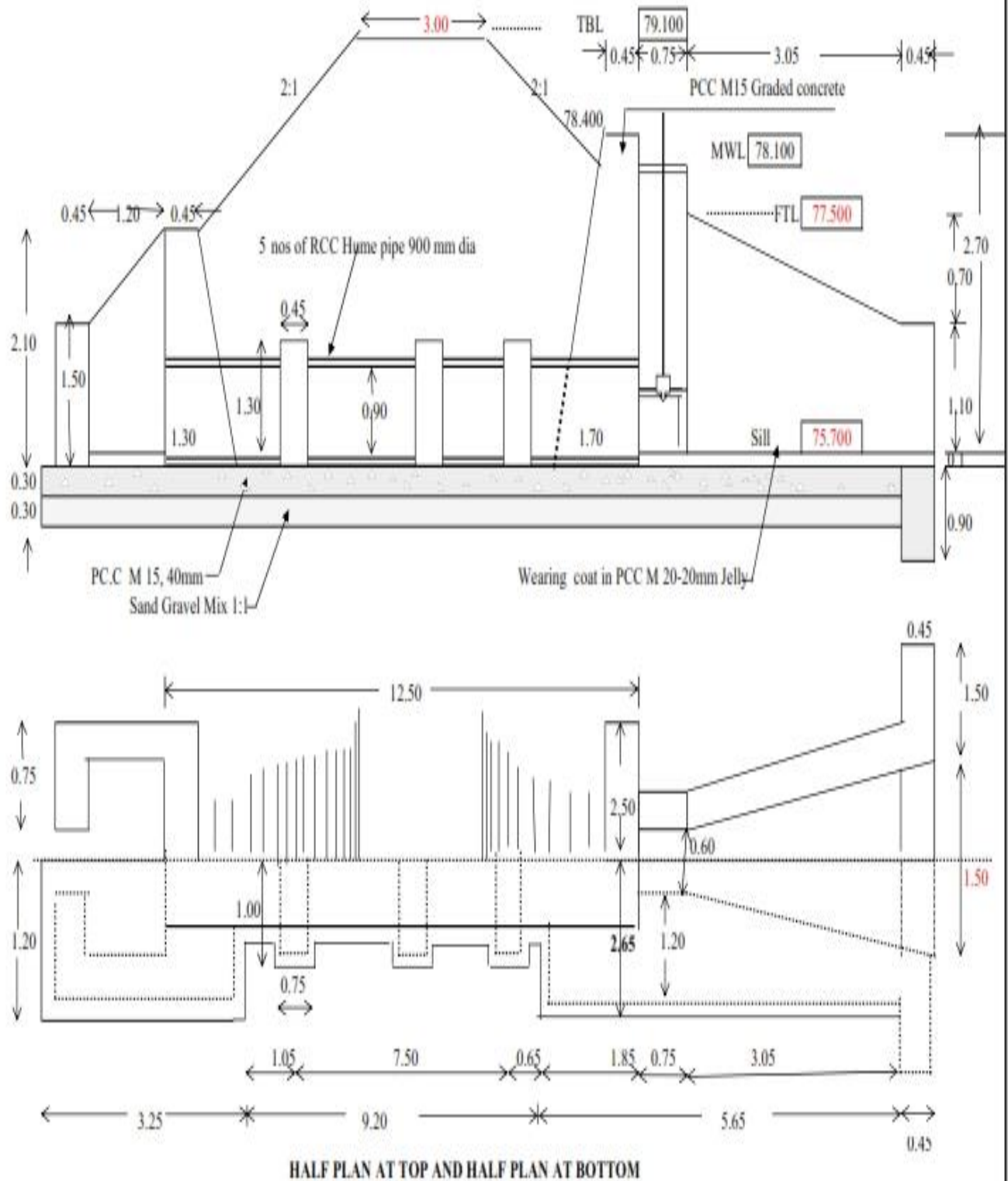
TYPICAL SECTION FOR SLUICE
