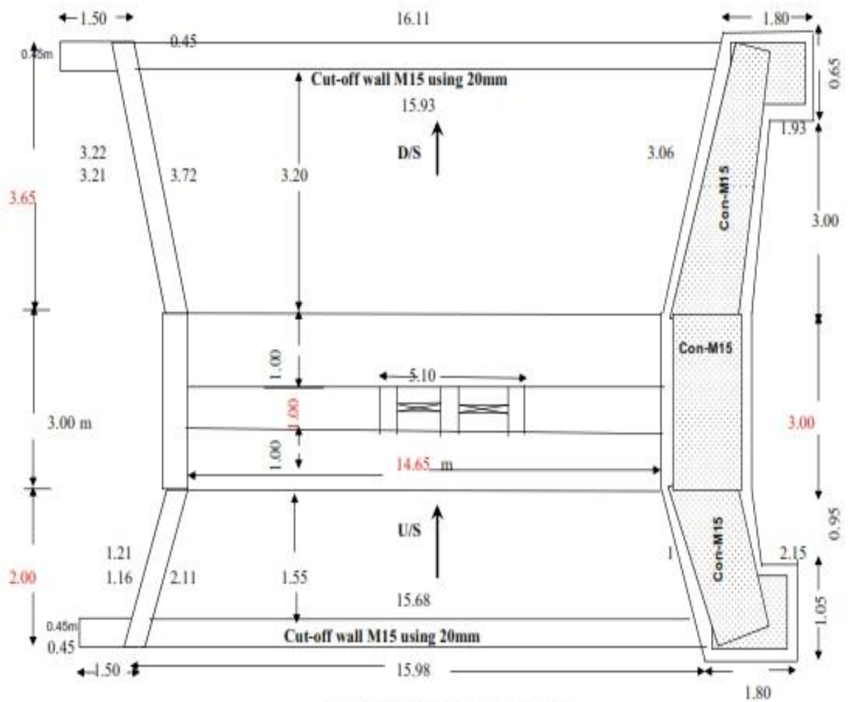
HALF SECTIONAL PLAN
