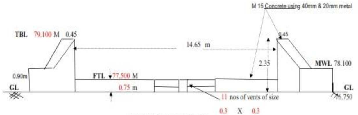
HALF SECTIONAL PLAN
