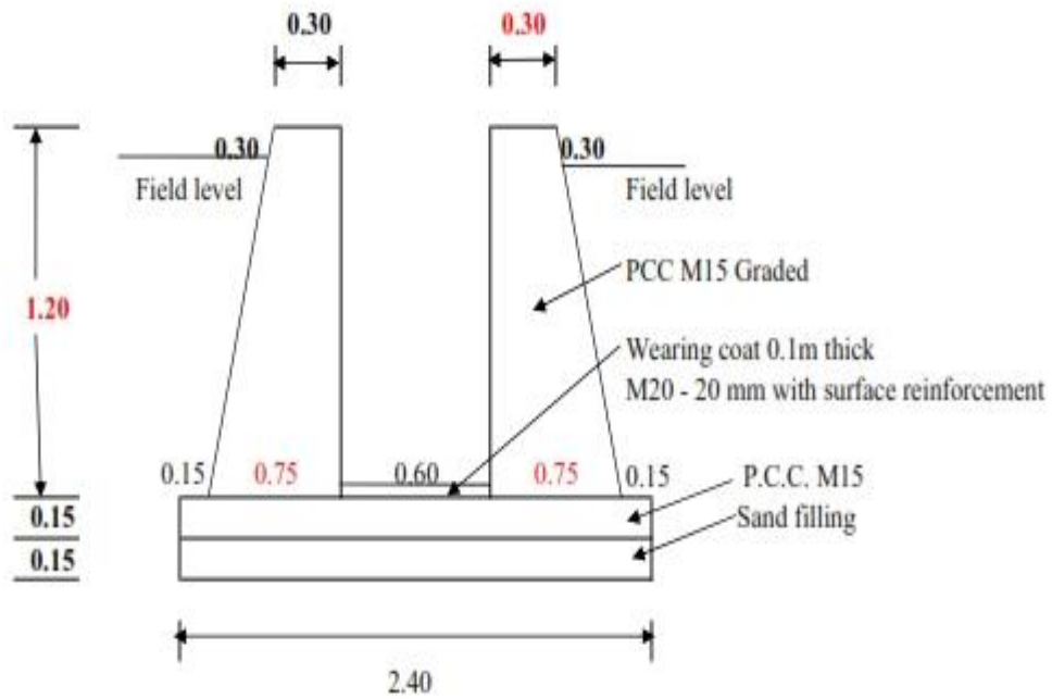
TYPICAL SECTION FOR FIELD CHANNEL
