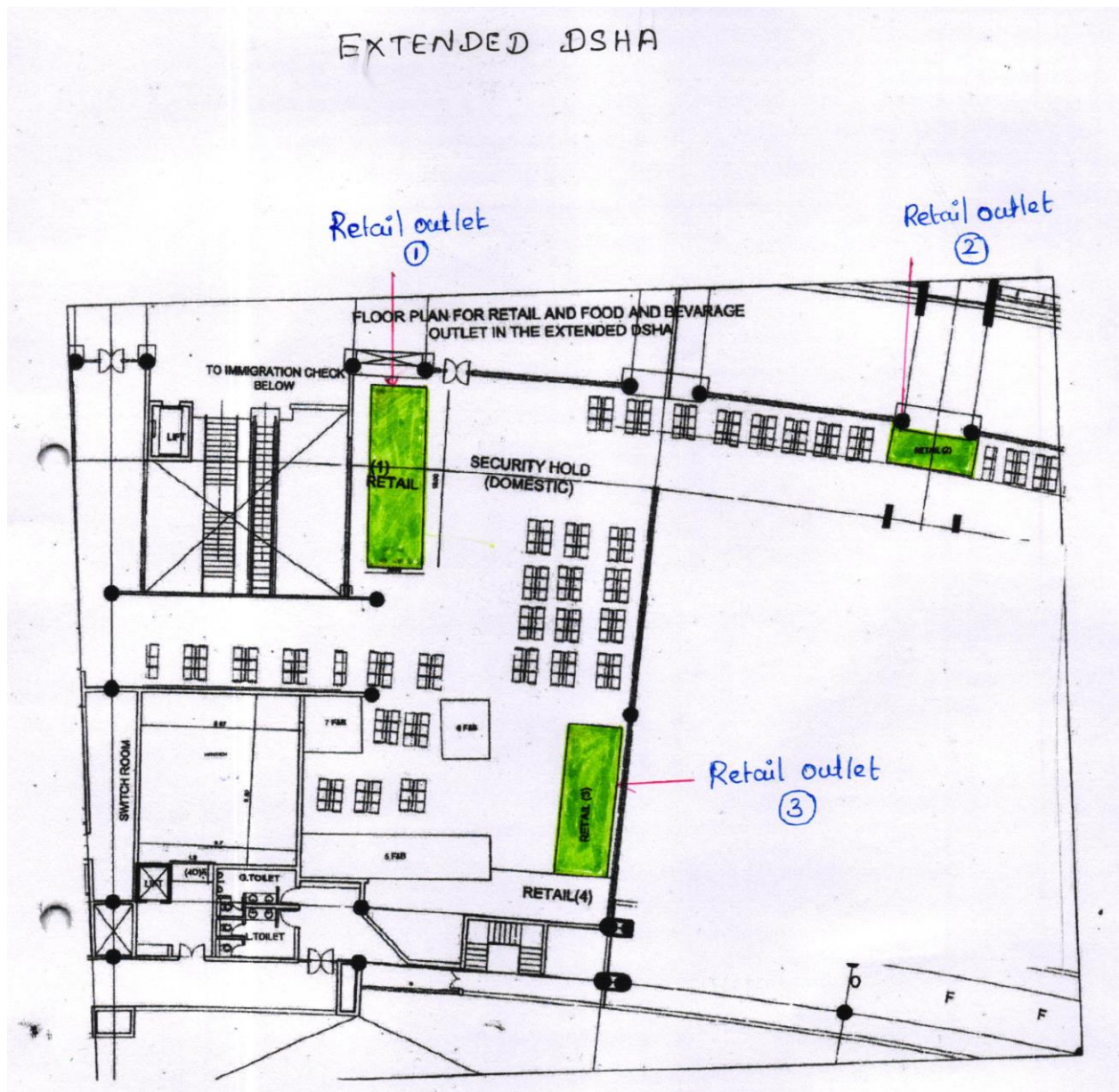
TERMINAL BUILDING – GROUND FLOOR
