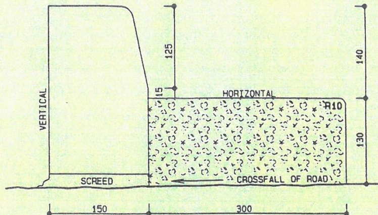
PRECAST BARRIER KERB AND CAST-IN-SITU CHANNEL
