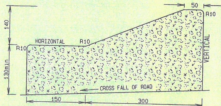
TYPICAL SECTION OF RESIDENTIAL ROAD SHOWING TYPE 1 MOUNTABLE KERB AND CHANNEL
