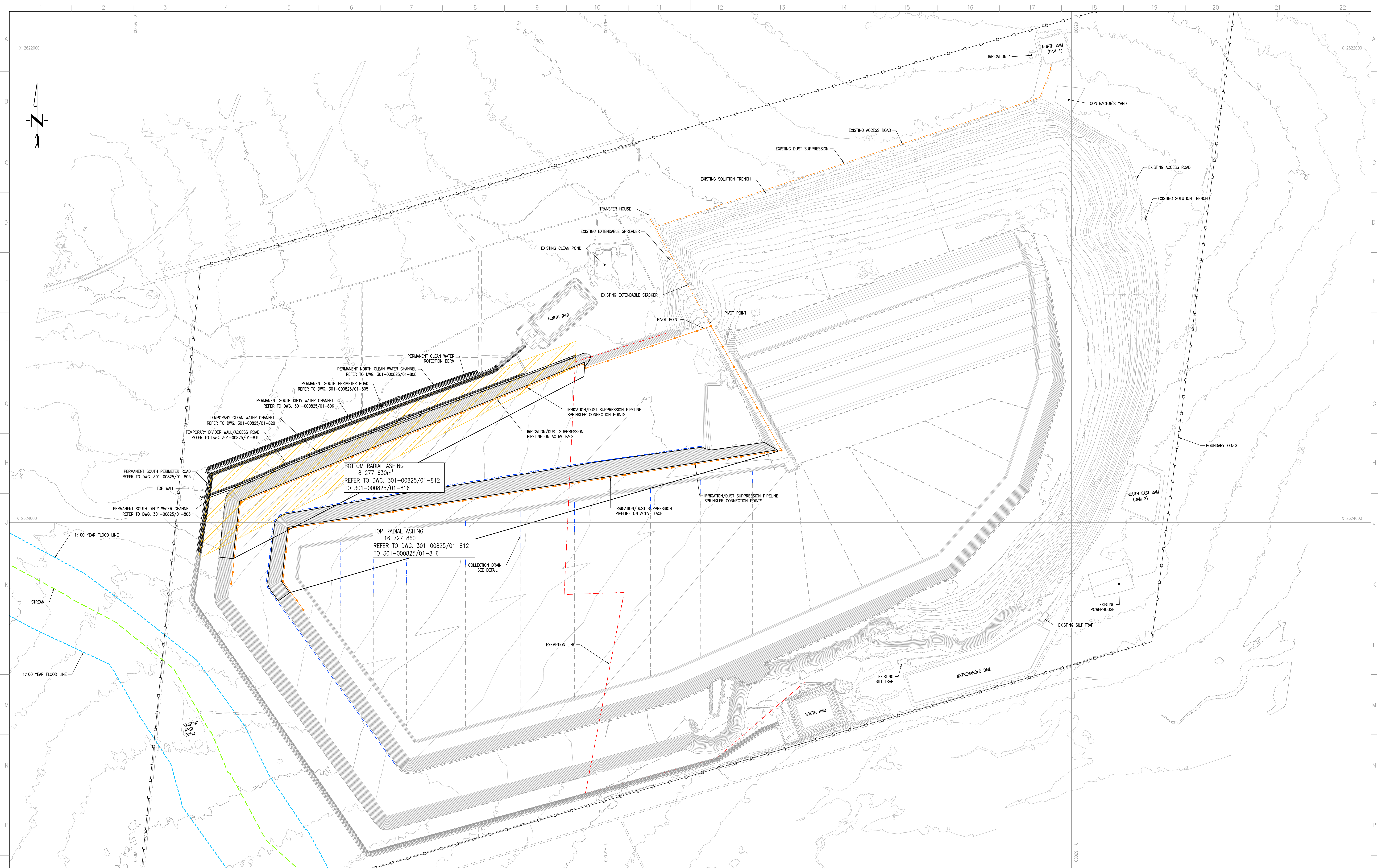
PHASE 8 (32 YEARS LINED AREA) LAYOUT PLAN SCALE 1:5000
