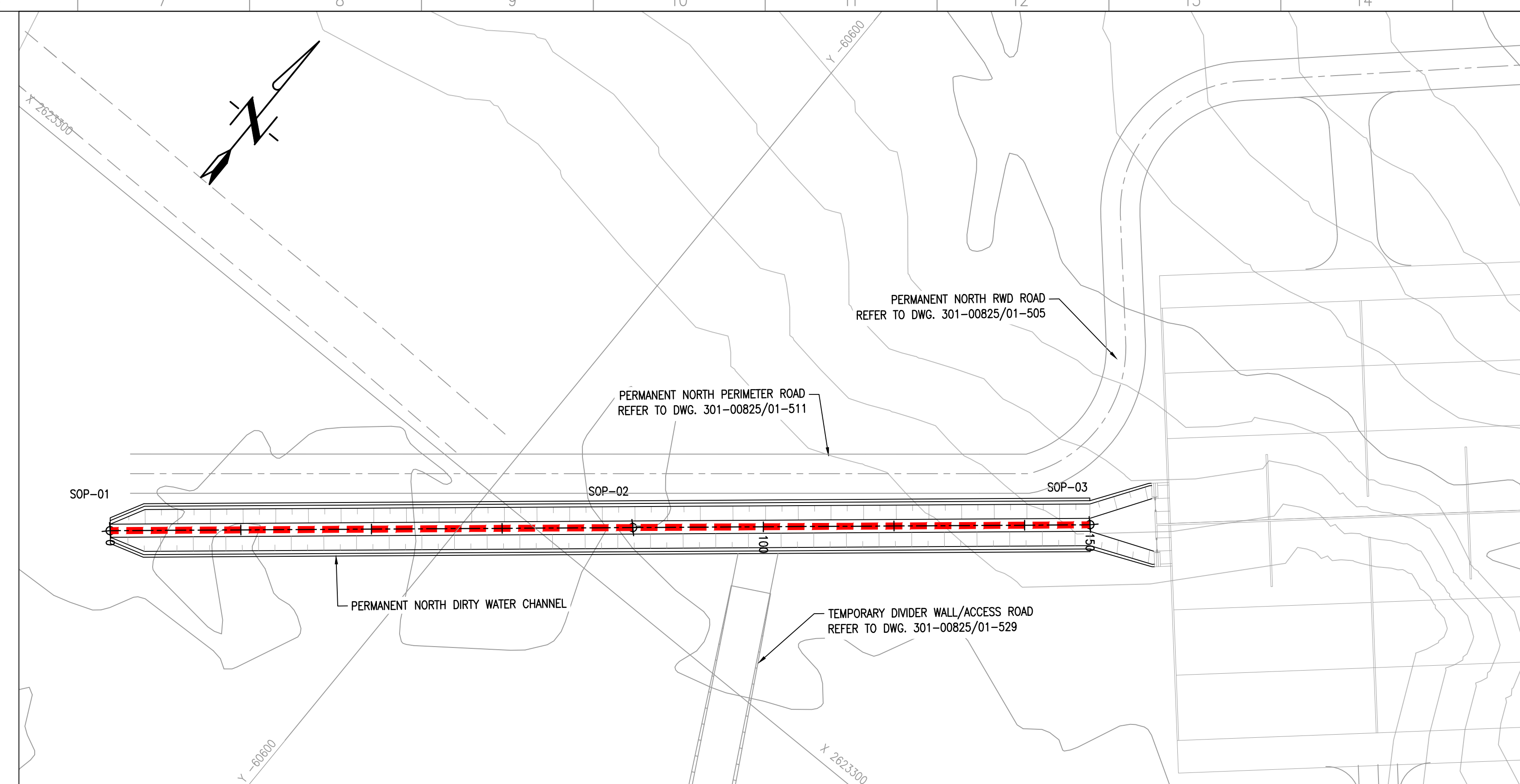
PERMANENT NORTH DIRTY WATER CHANNEL LAYOUT PLAN SCALE 1:2000
