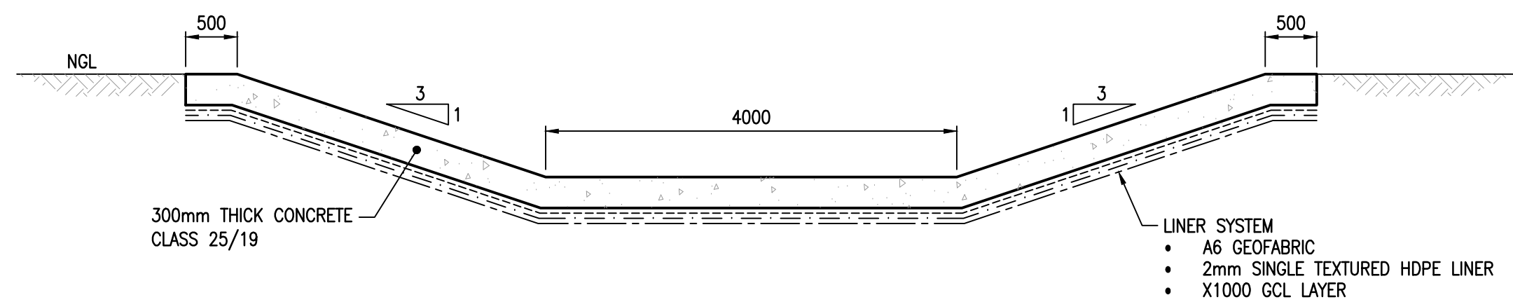
TYPICAL SECTION SCALE 1:50
