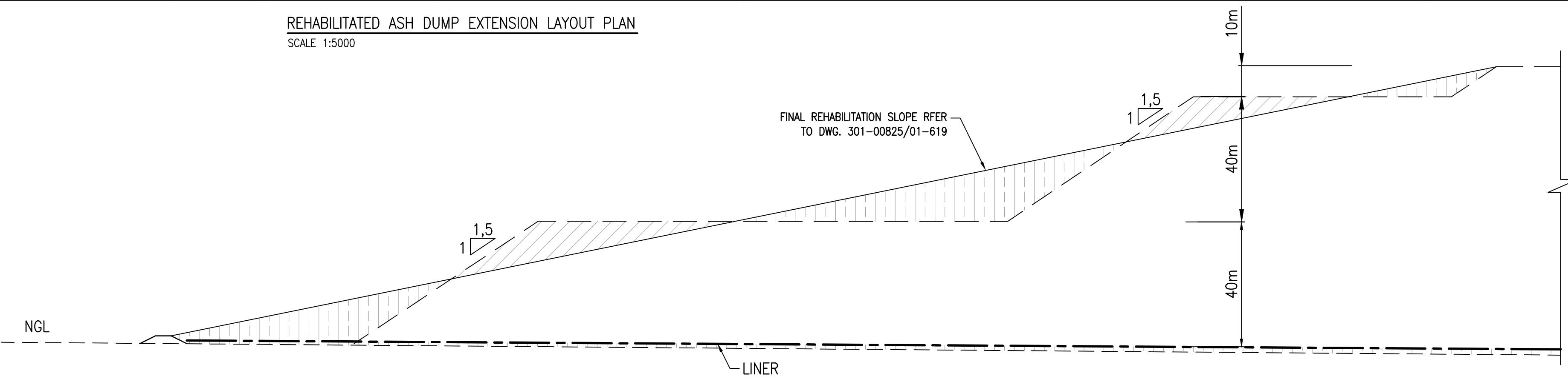
TYPICAL SECTION B-B
