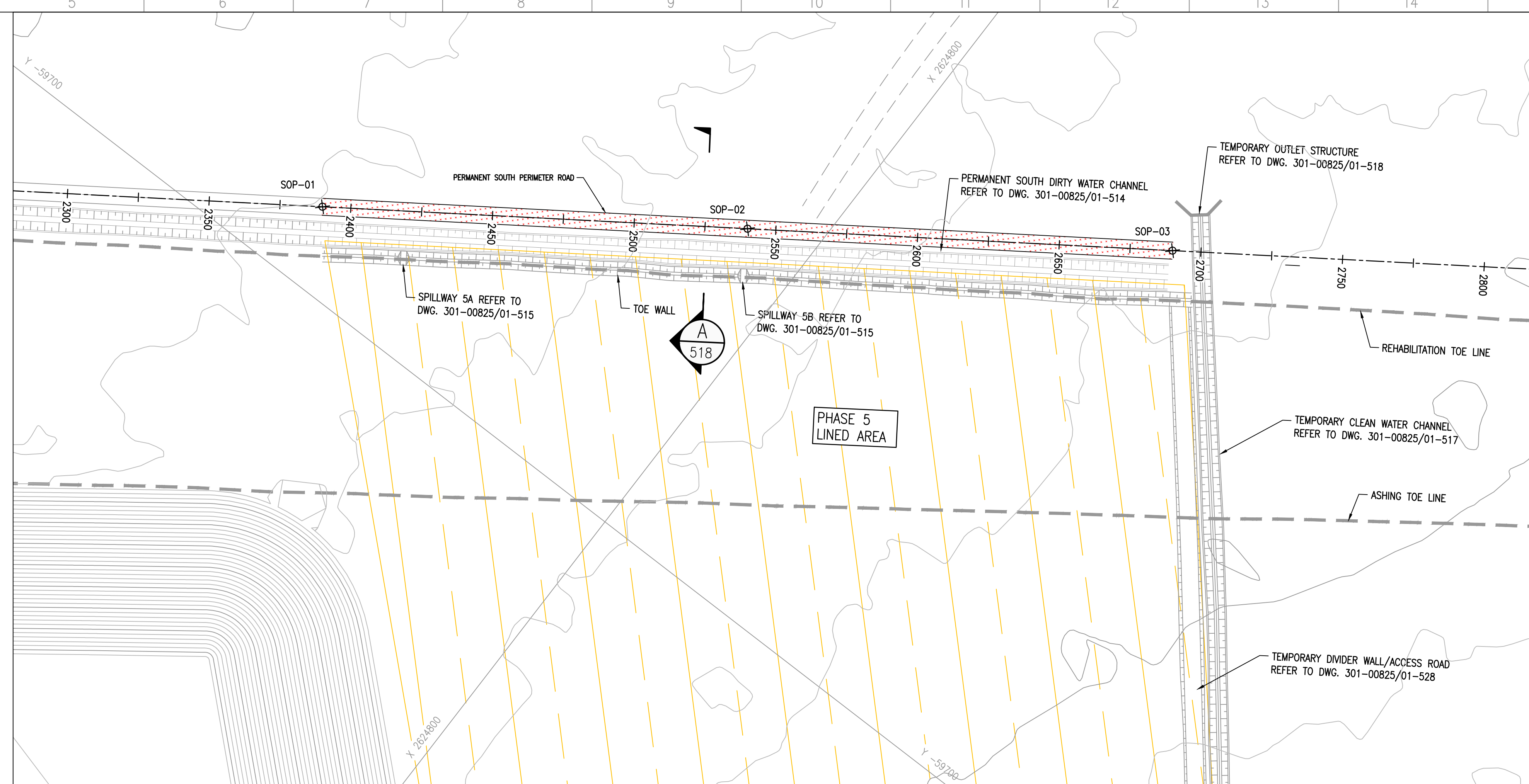
PERMANENT SOUTH PERIMETER ROAD LAYOUT PLAN SCALE 1:1000
