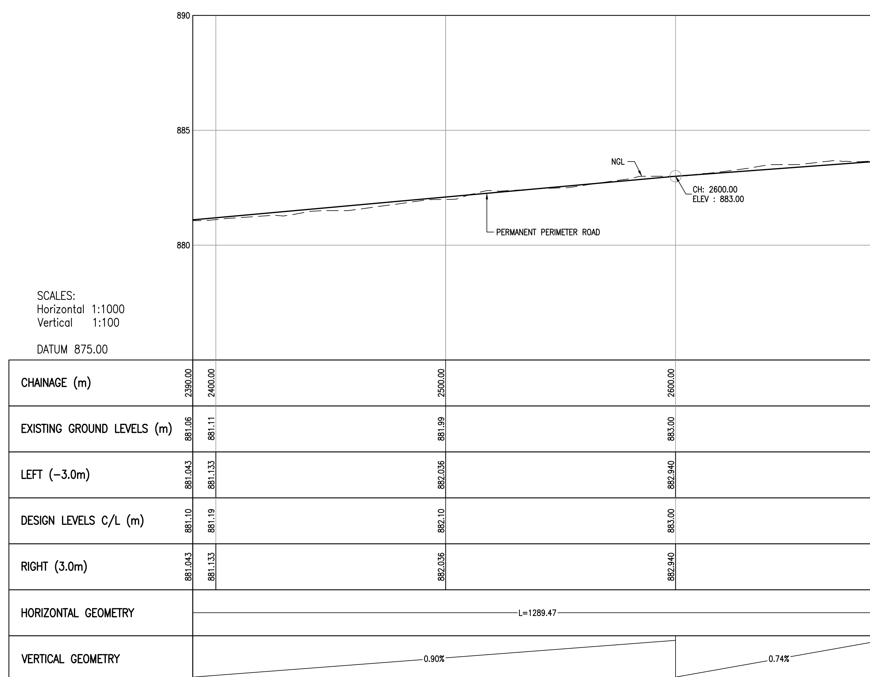
PERMANENT SOUTH PERIMETER ROAD CH. 2390 - CH. 2690 SCALE 1:1000
