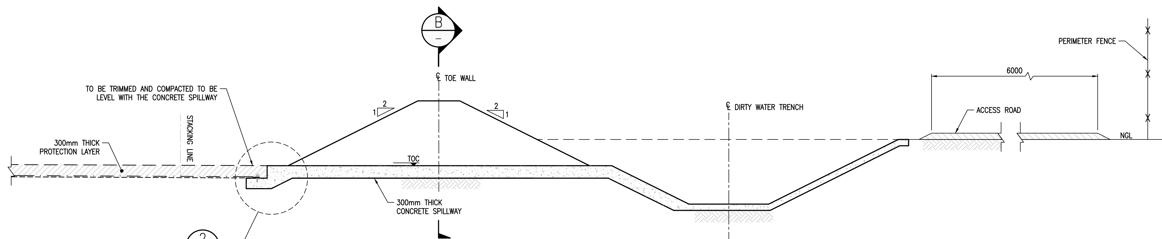
A TYPICAL WEIR SECTION SCALE 1:50
