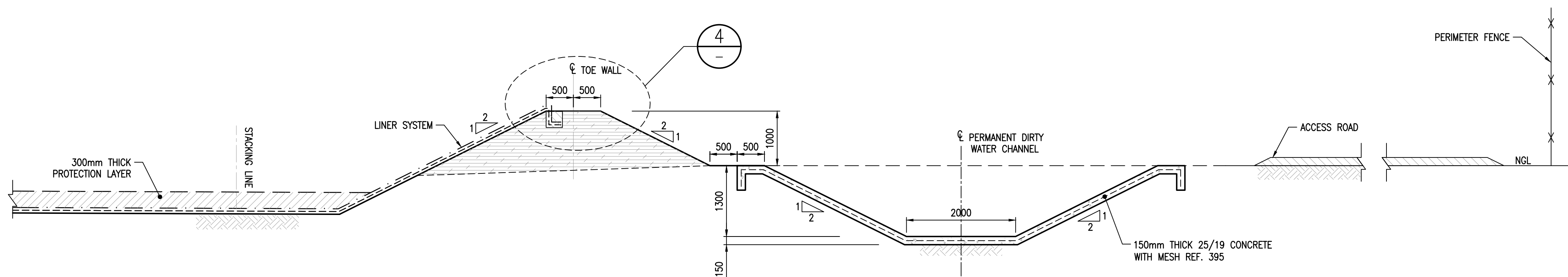
C TYPICAL TOE WALL SECTION SCALE 1:50
