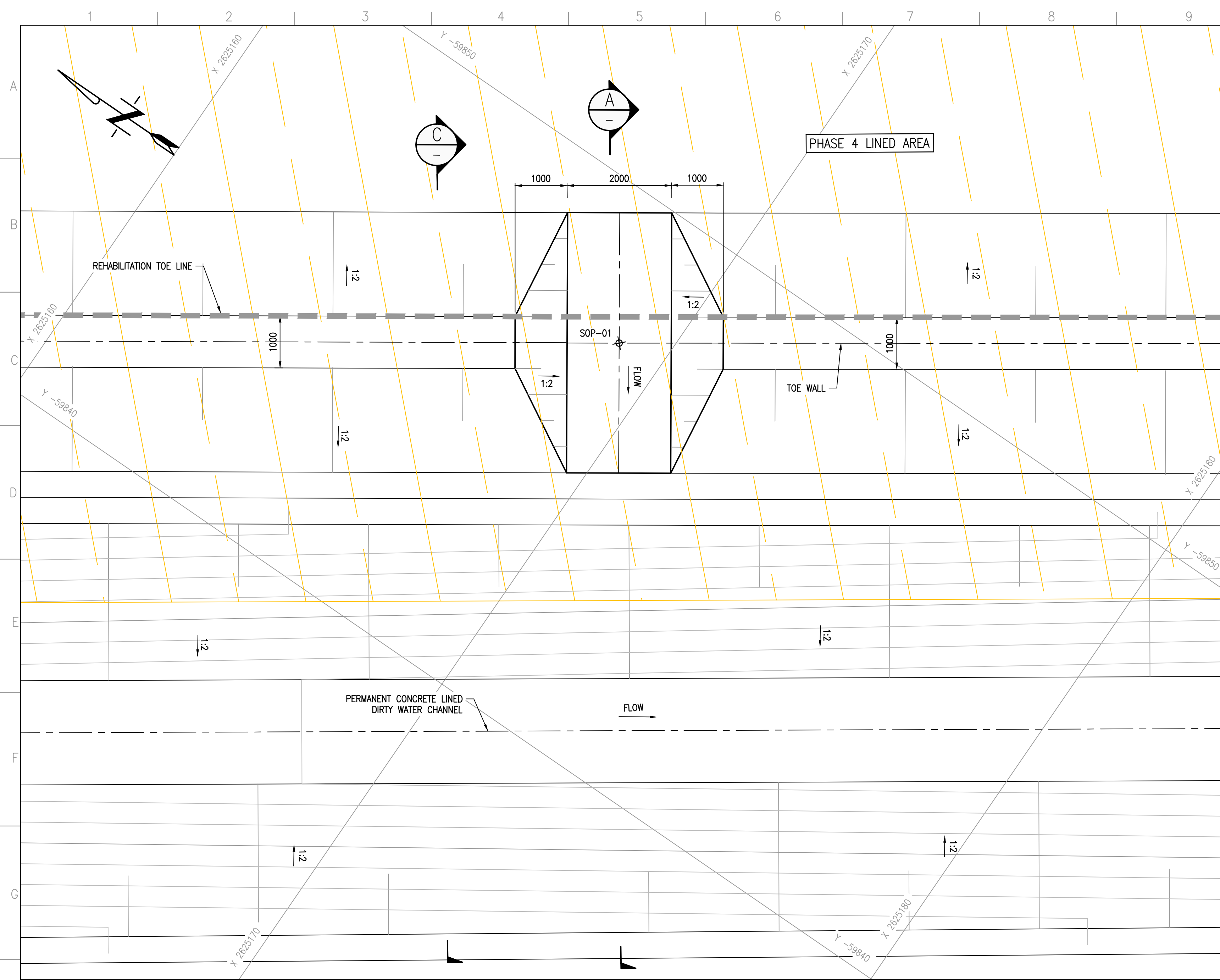
1 SPILLWAY 4A LAYOUT PLAN SCALE 1:50
