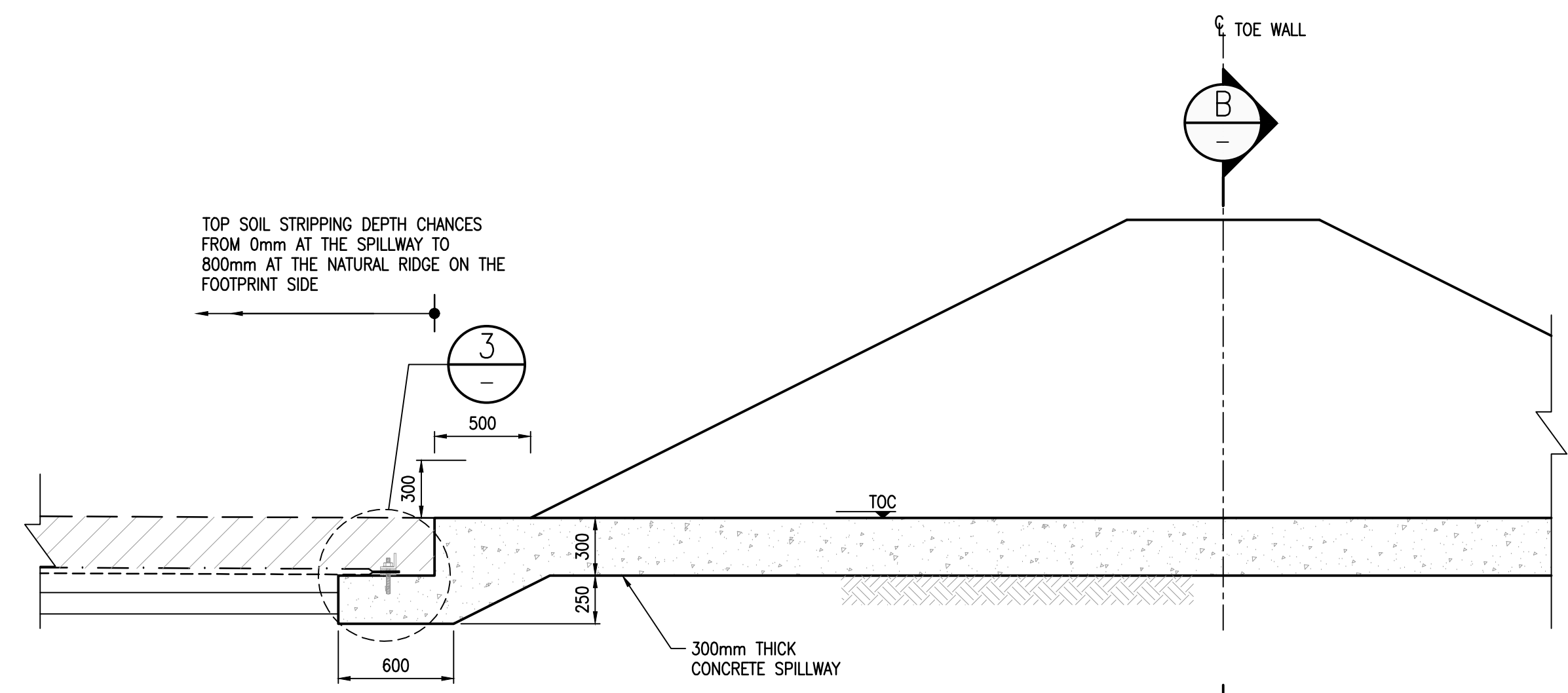
2 TYPICAL DETAIL SCALE 1:25
