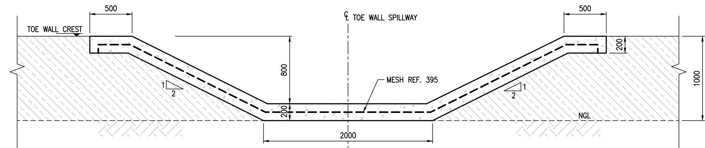
B TYPICAL SPILLWAY SECTION SCALE 1:25
