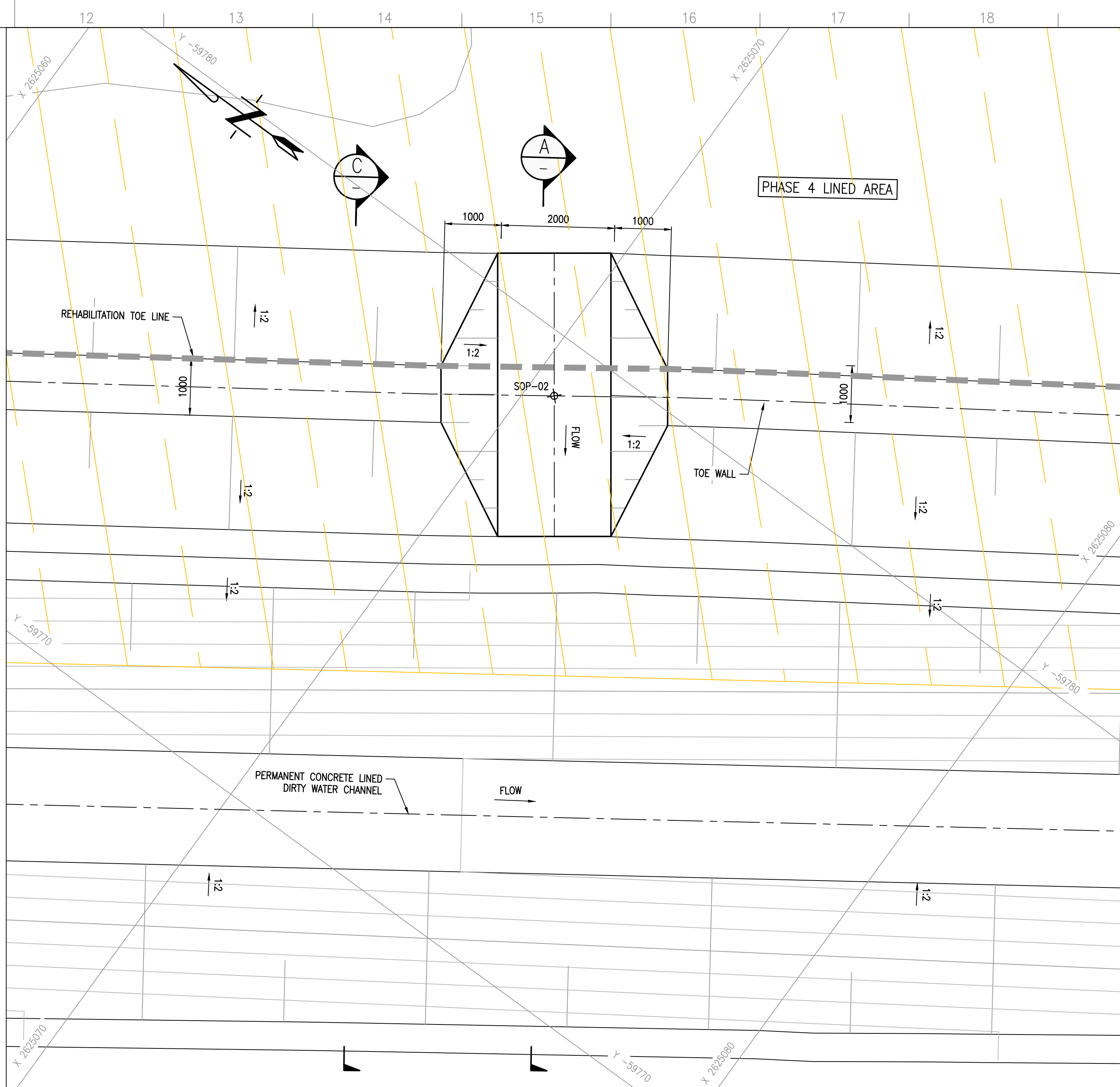
2 SPILLWAY 4B LAYOUT PLAN SCALE 1:50
