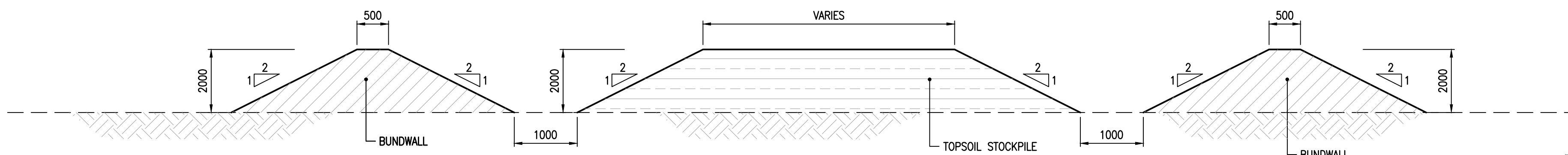
A TYPICAL STOCKPILE SECTION SCALE 1:50
