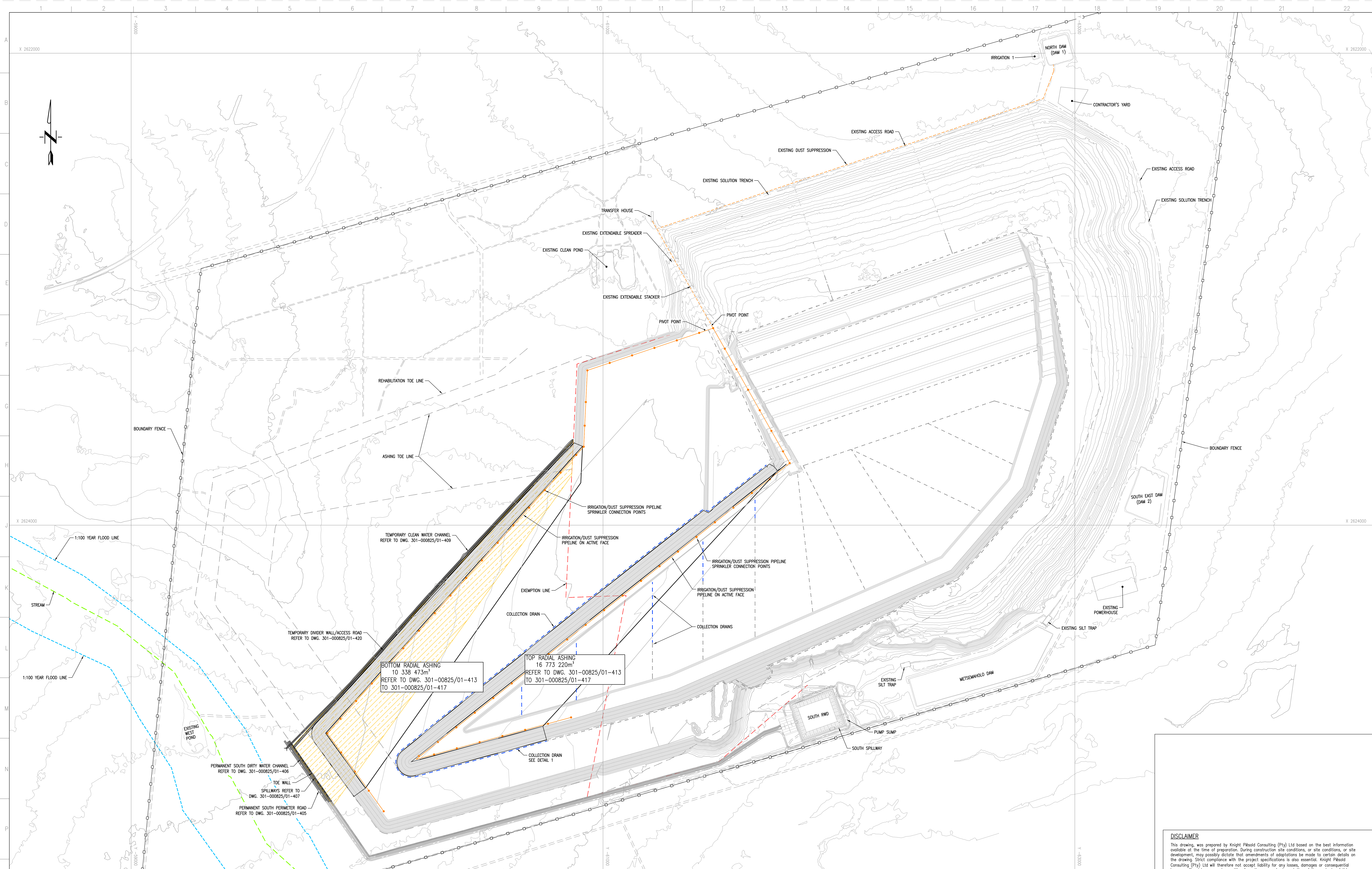
PHASE 4 (16 YEARS LINED AREA) LAYOUT PLAN SCALE 1:5000
