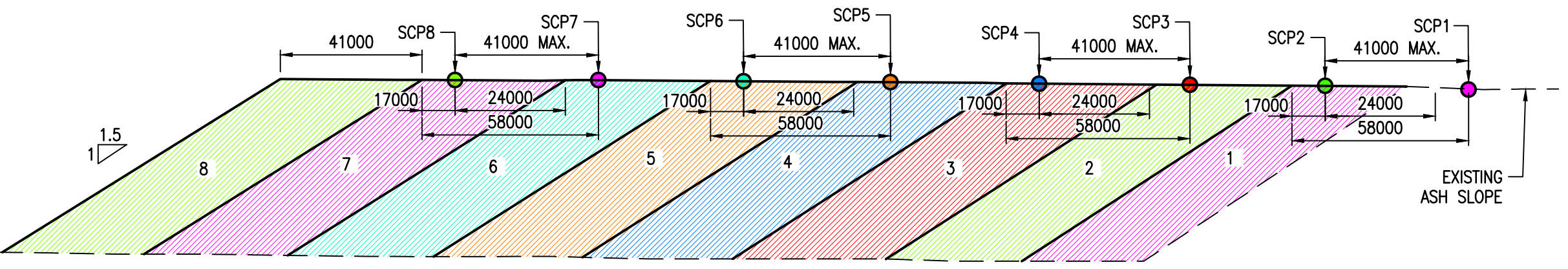
MCP9 TO MCP23 AND SCP1 TO SCP9 POSITIONS LAYOUT PLAN SCALE 1:5000
