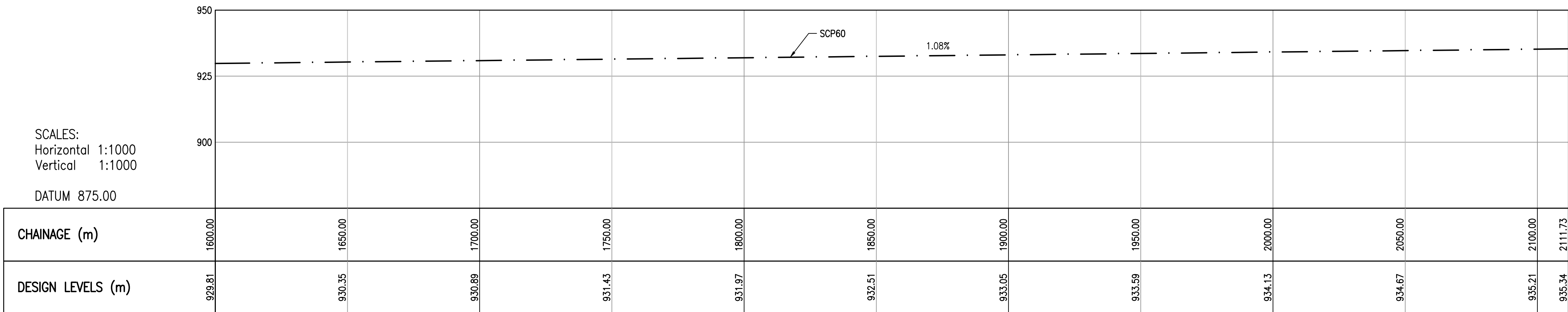
SCP60 LONGITUDINAL SECTION CH. 1600 TO CH. 2111.73 SCALE 1:1000
