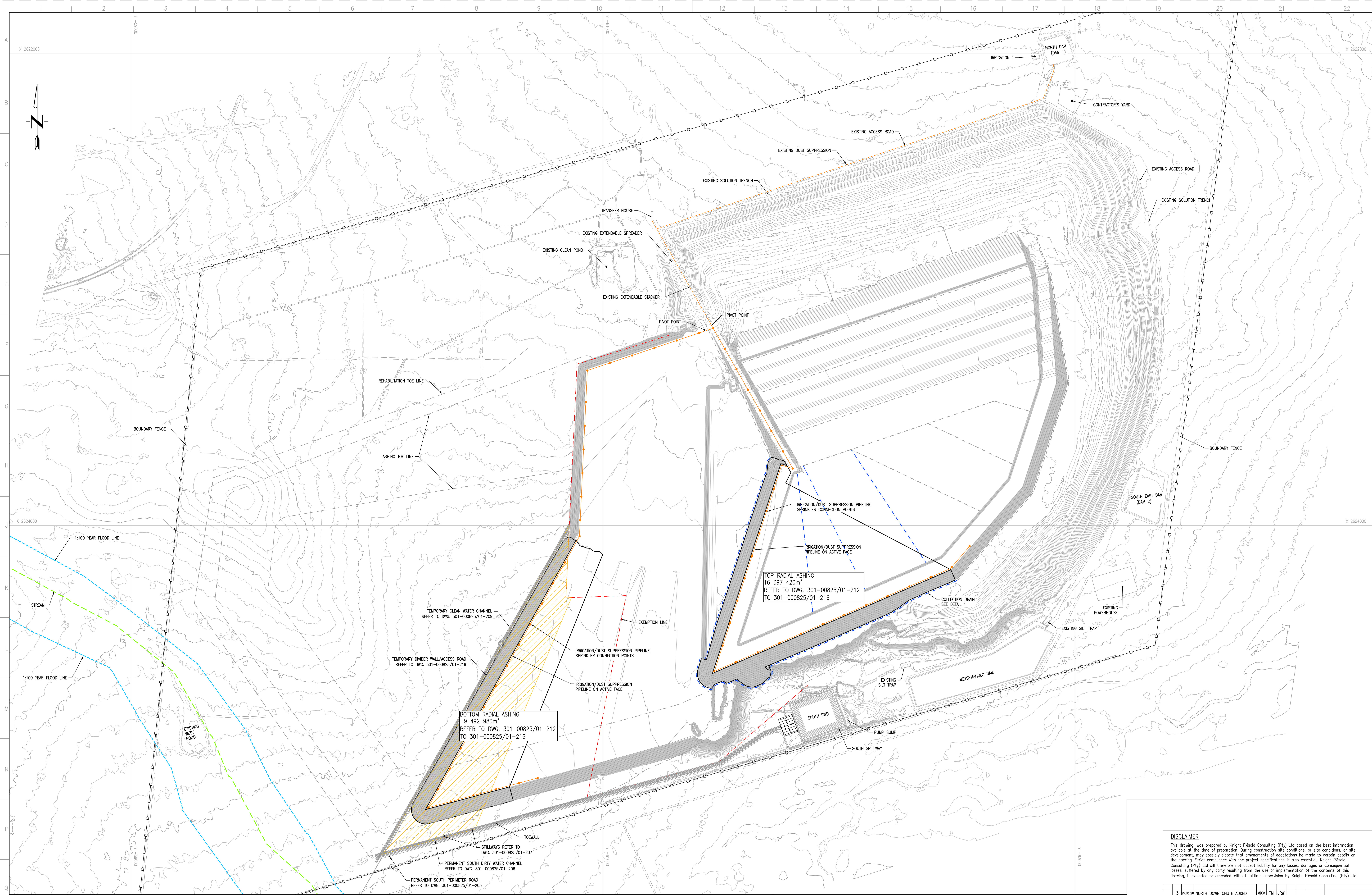
PHASE 2 (8 YEARS LINED AREA) LAYOUT PLAN SCALE 1:5000
