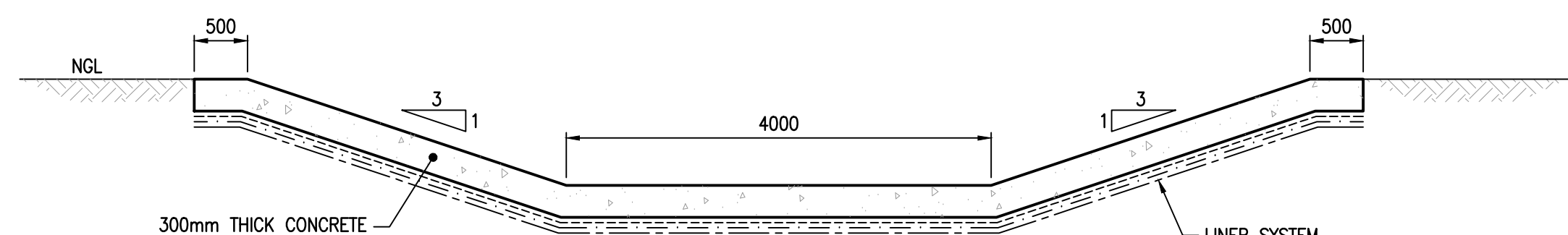
B TYPICAL SECTION SCALE 1:50
