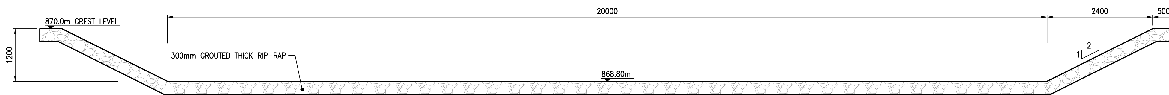
A SPILLWAY SECTION SCALE 1:50
