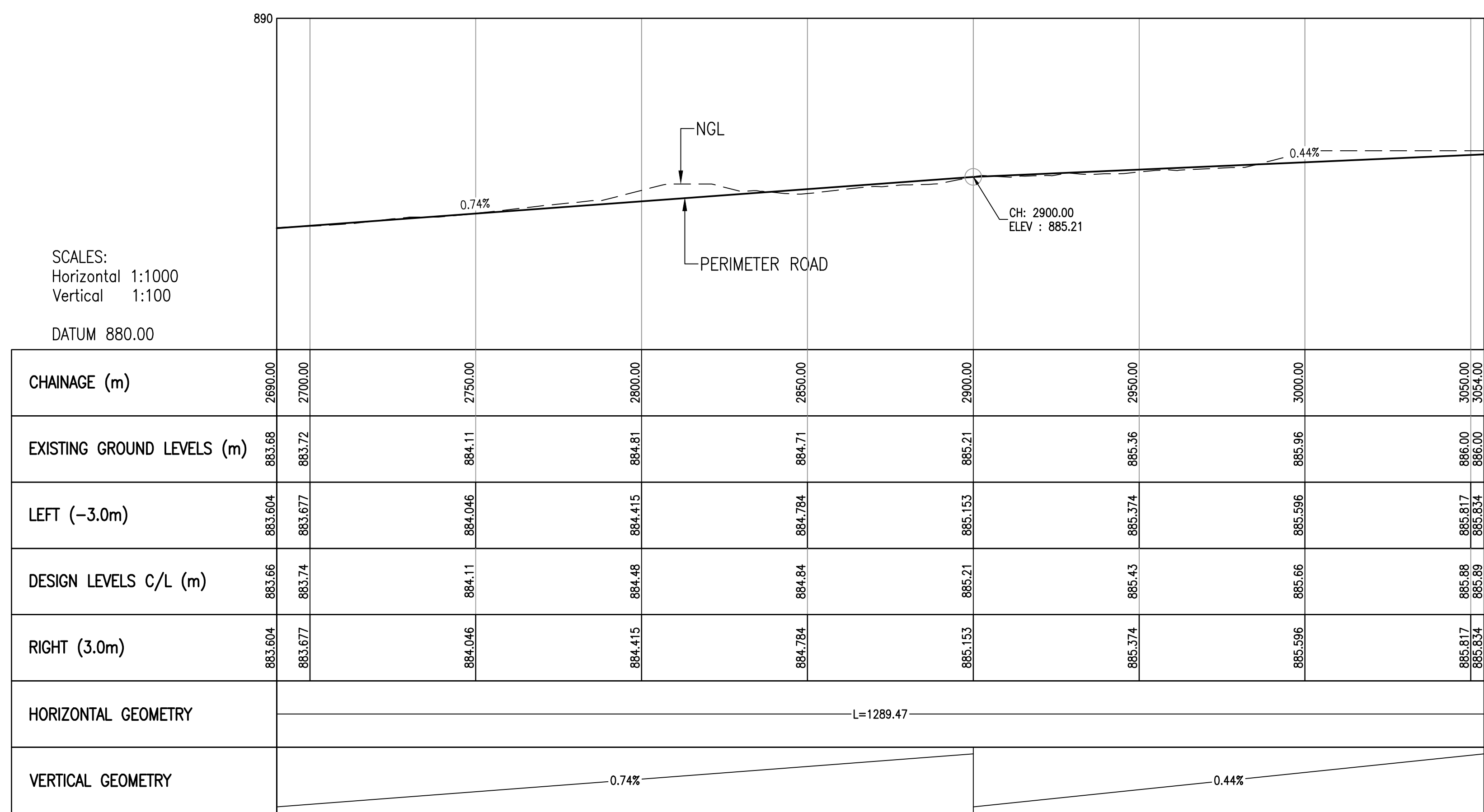
PERMANENT SOUTH PERIMETER ROAD LONGITUDINAL SECTION CH. 2690 - CH. 3040 SCALE 1:1000
