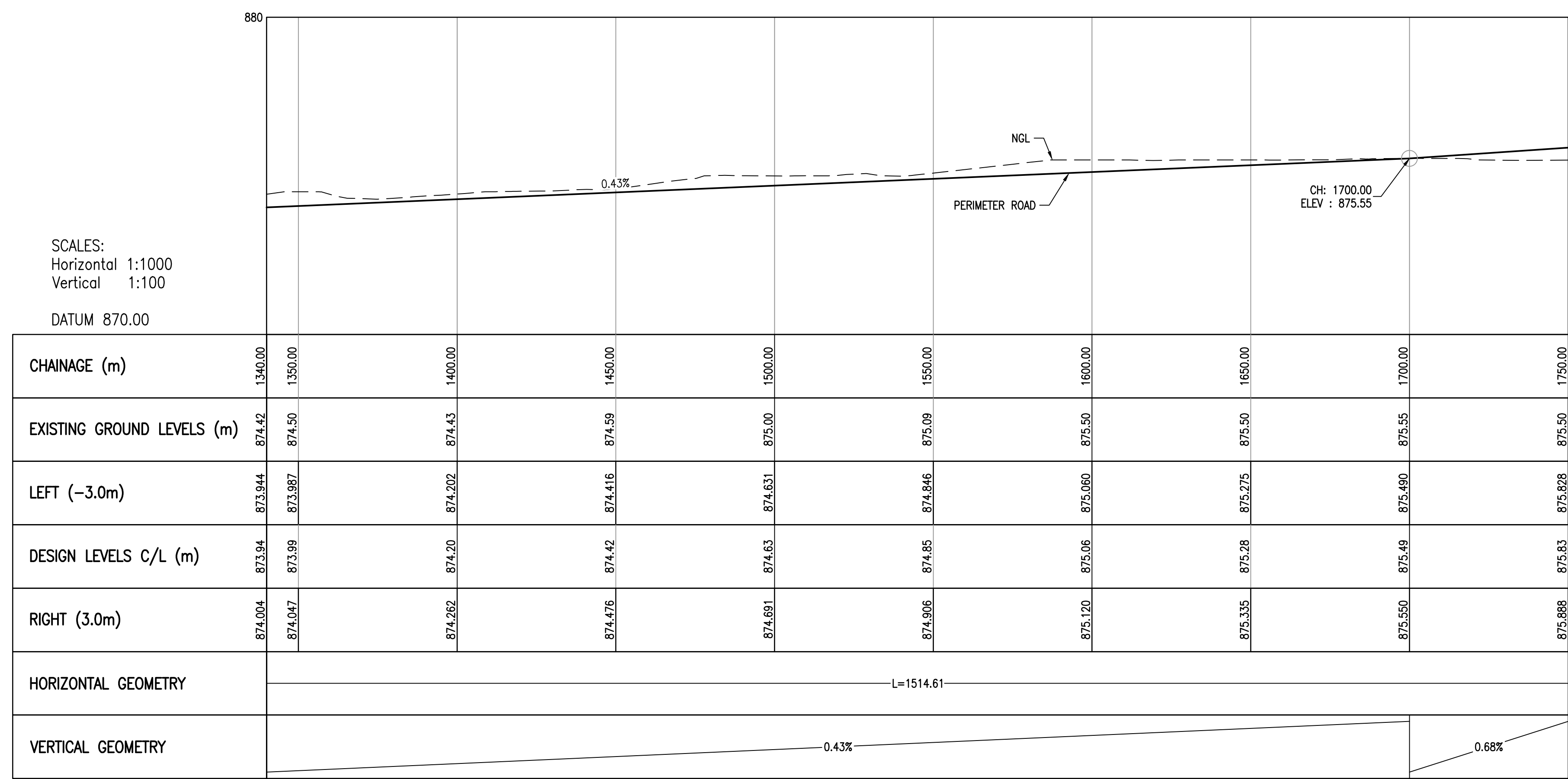
PERMANENT SOUTH PERIMETER ROAD CH. 1340 - CH. 1750 SCALE 1:1000
