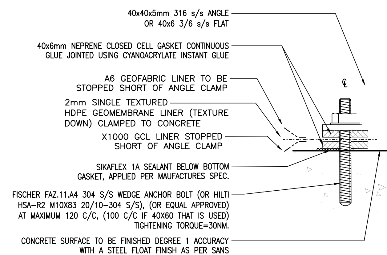
3 LINER SYSTEM FIXING DETAIL SCALE 1:2
