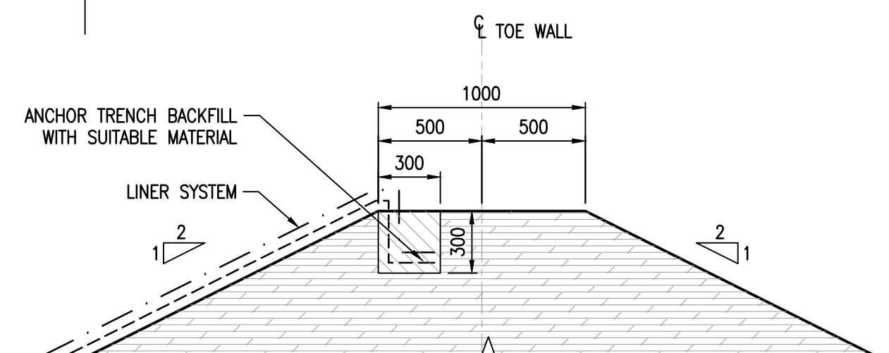
4 ANCHOR TRENCH — SCALE 1:25
