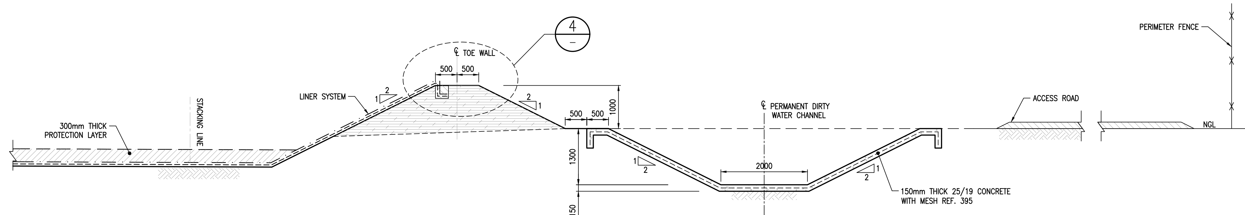
C TYPICAL TOE WALL SECTION SCALE 1:50
