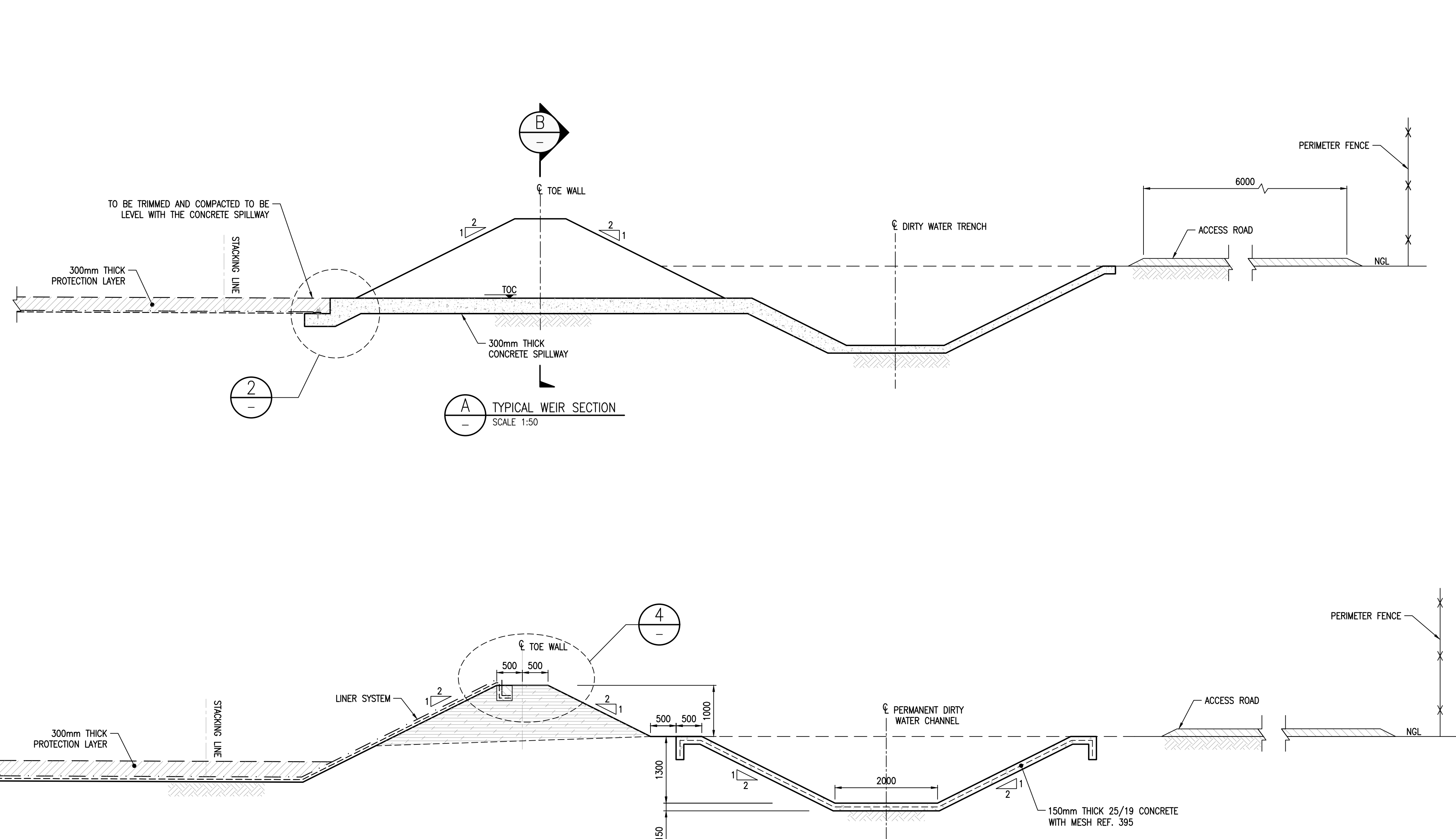
C TYPICAL TOE WALL SECTION SCALE 1:50
