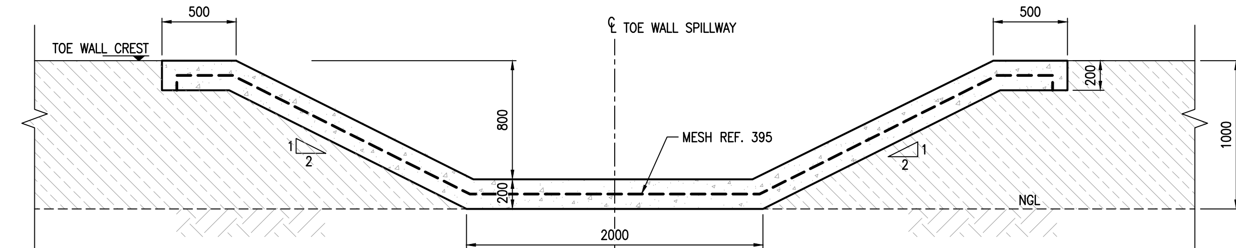
B TYPICAL SPILLWAY SECTION SCALE 1:25
