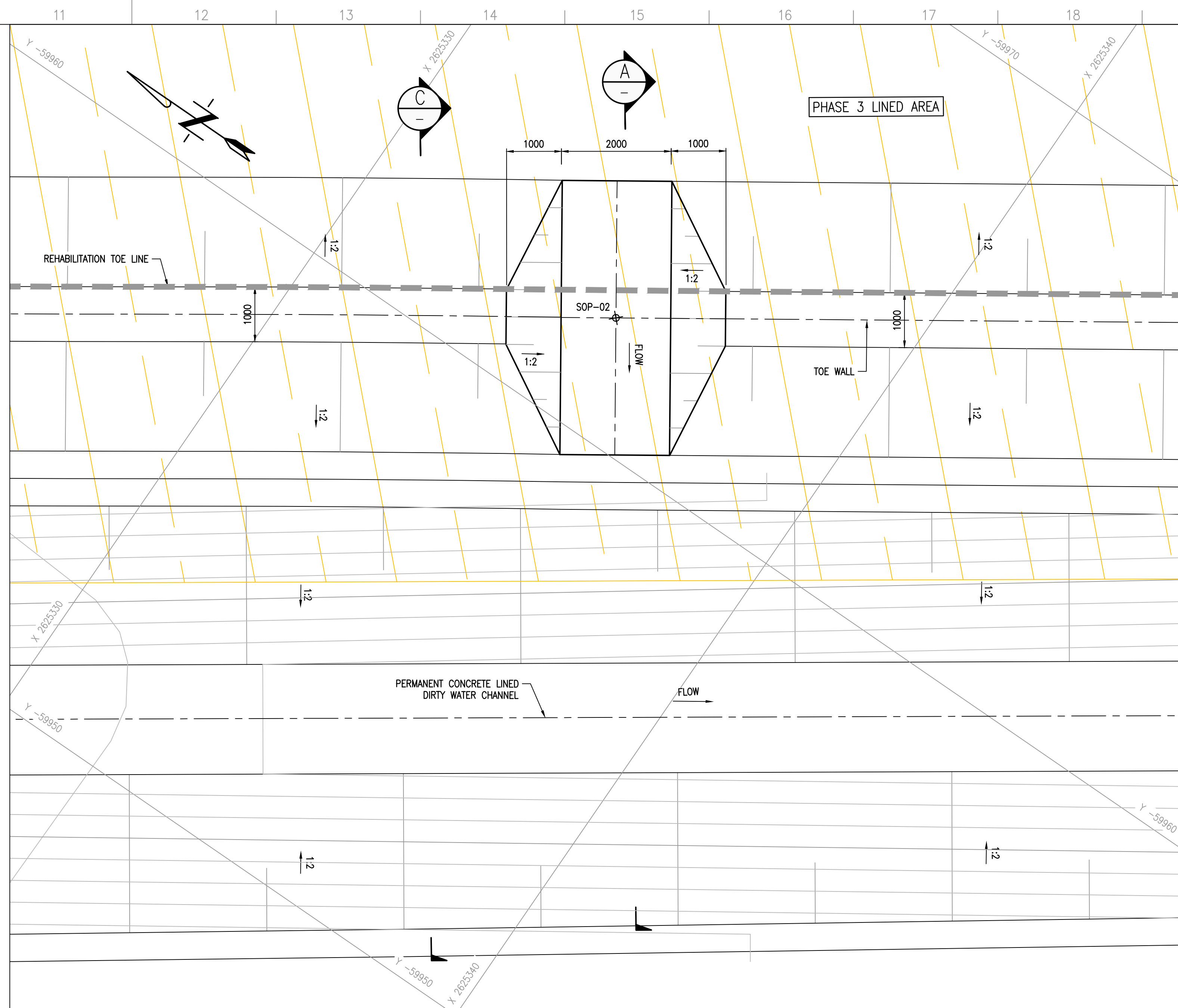
2 SPILLWAY 3B LAYOUT PLAN SCALE 1:50
