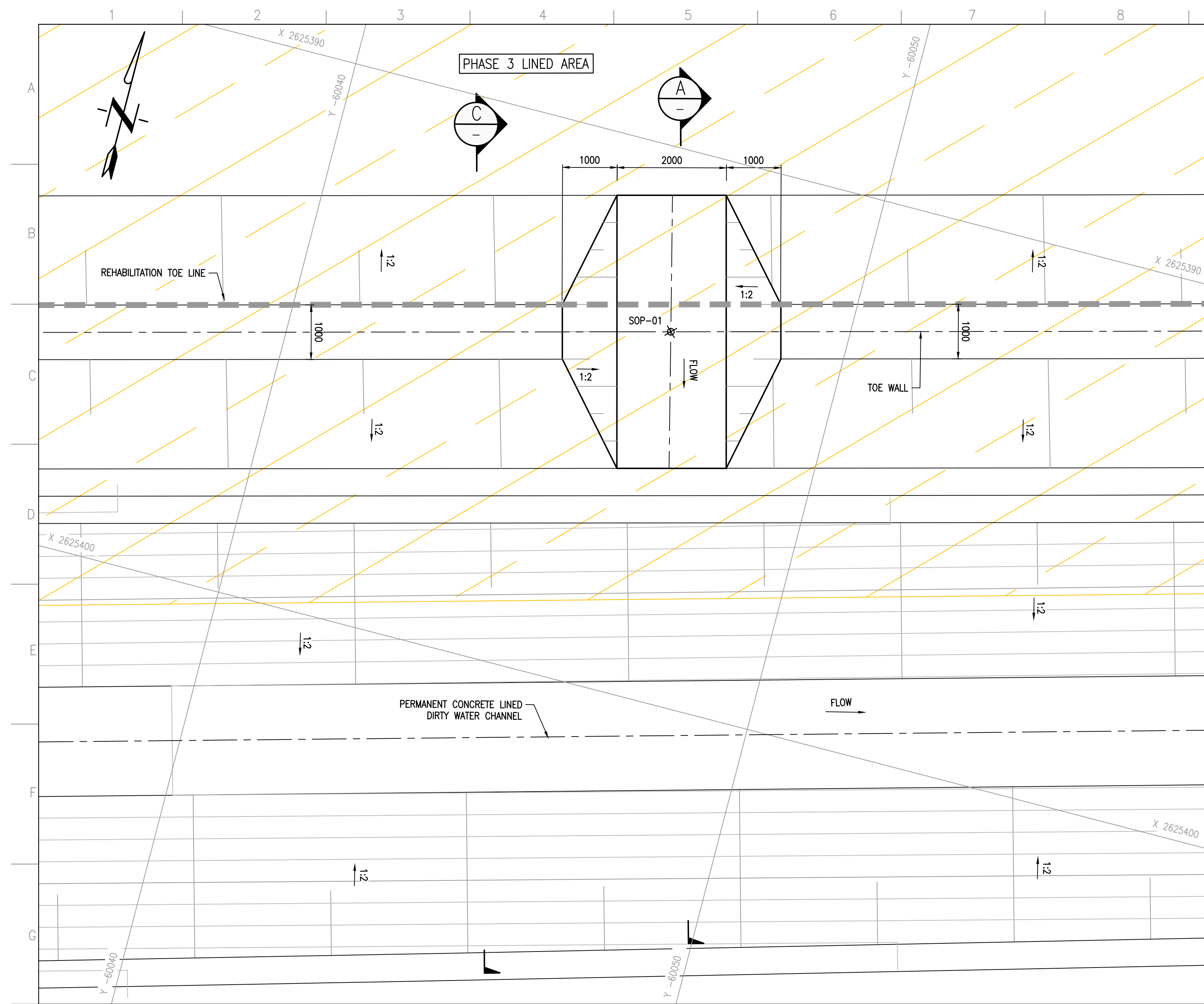
1 SPILLWAY 3A LAYOUT PLAN SCALE 1:50
