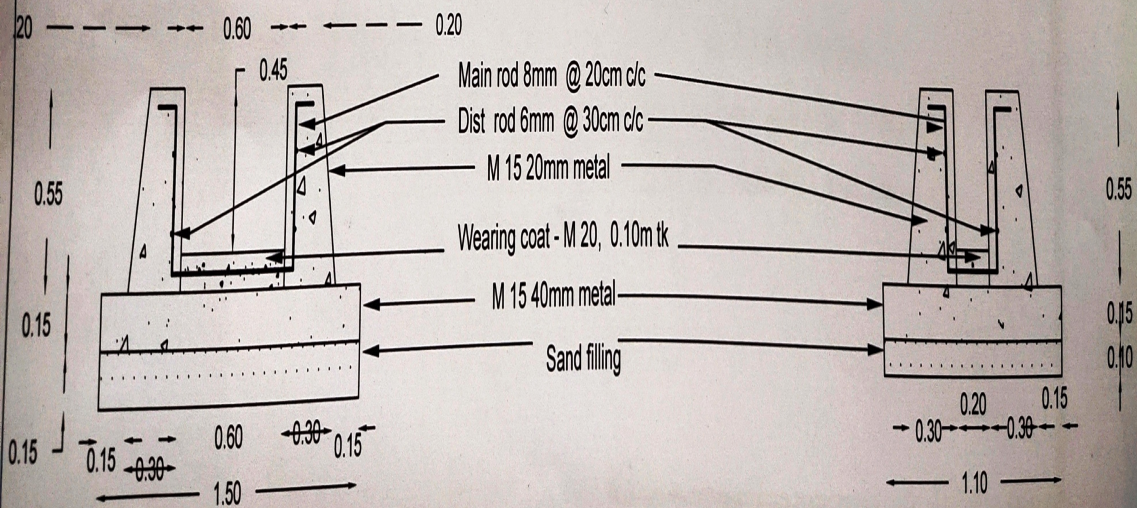
CROSS SECTION AT BB
