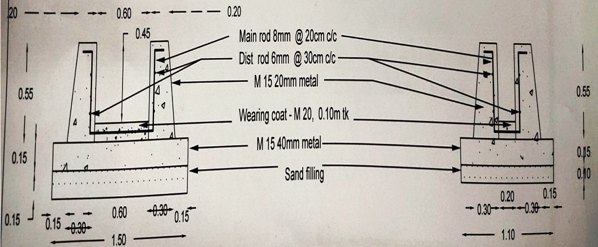
CROSS SECTION AT BB
