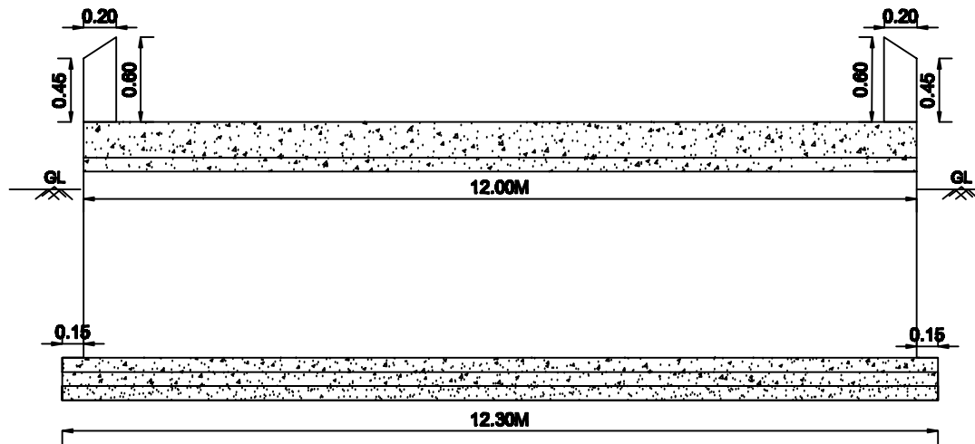
LONGITUDINAL SECTION OF CULVERT
