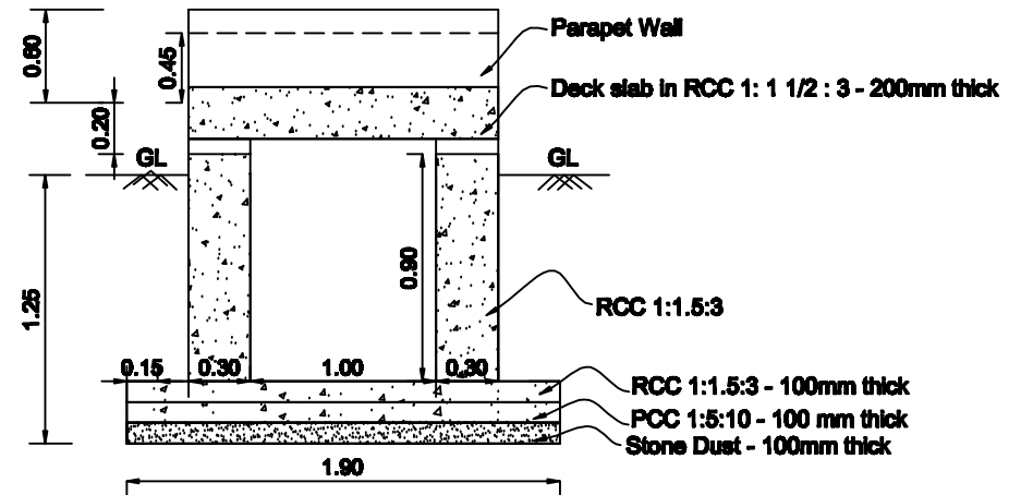
CROSS SECTION OF CULVERT
