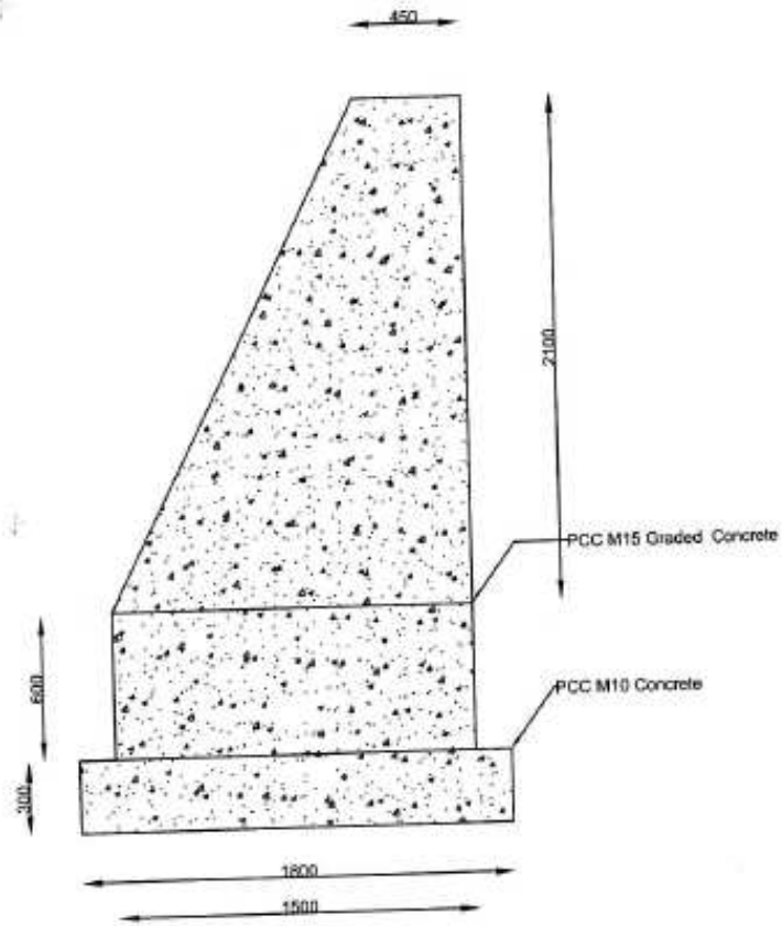
C/S of Retaining Wall
