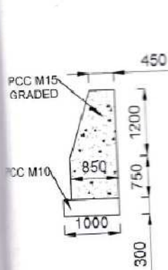
C/S of Return Wall
