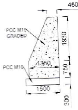
C/S of Wing Wall
