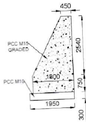
C/S of Guide Wall
