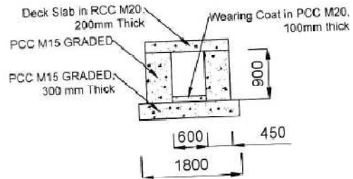
C/S of Barrel
