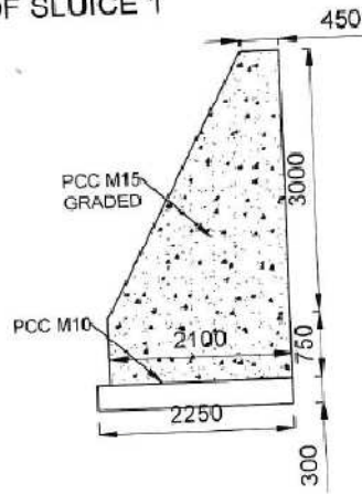
C/S of Guide Wall
