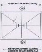
PLAN TYPICAL ISOLATED FOOTING DETAIL
