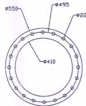
EXPANDER 300 X 350NB
