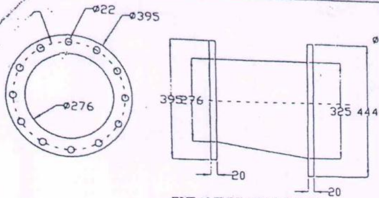
EXPANDER 250 X 300NB
