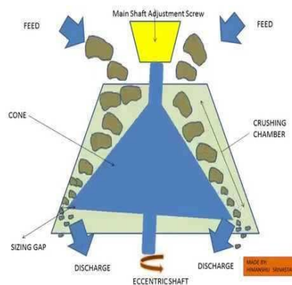
Cone Crusher
