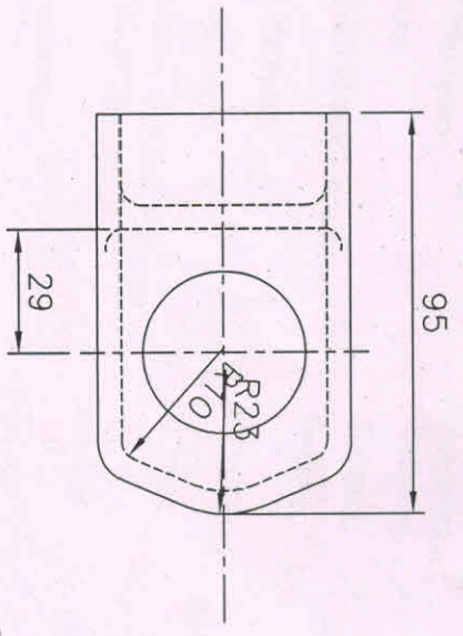
NOZZLE HEAD - PLAN
