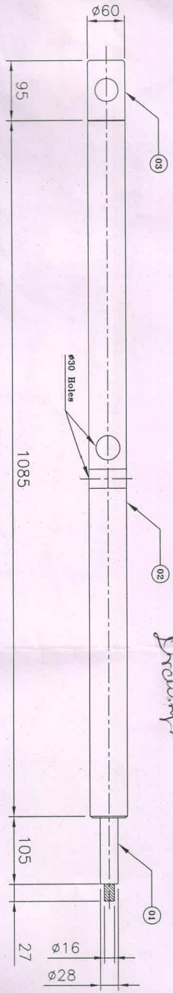
NOZZLE HEAD-ELEVATION
