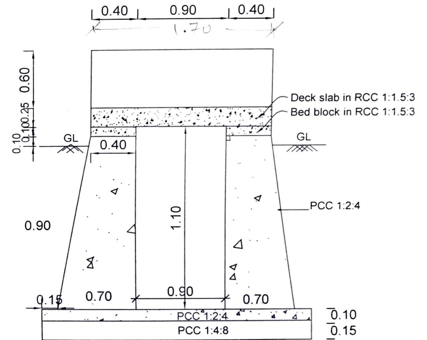
CROSS SECTION OF CULVERT
