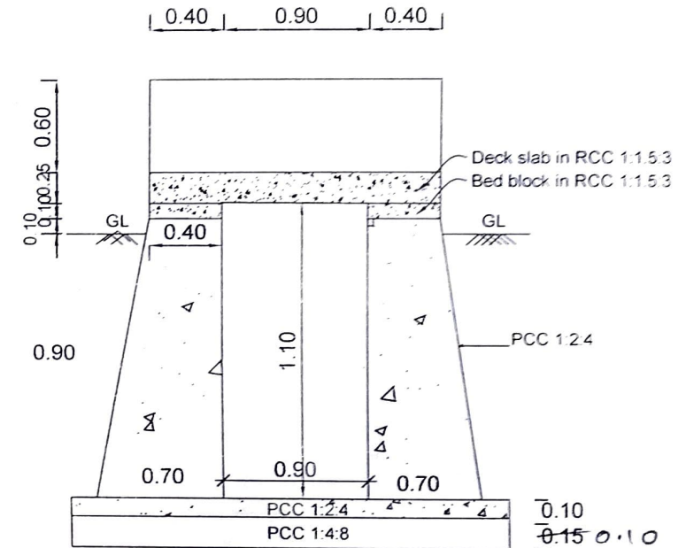
CROSS SECTION OF CULVERT
