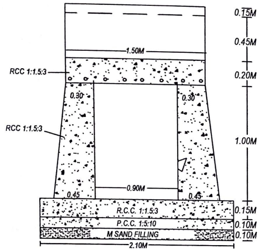
CROSS SECTION
