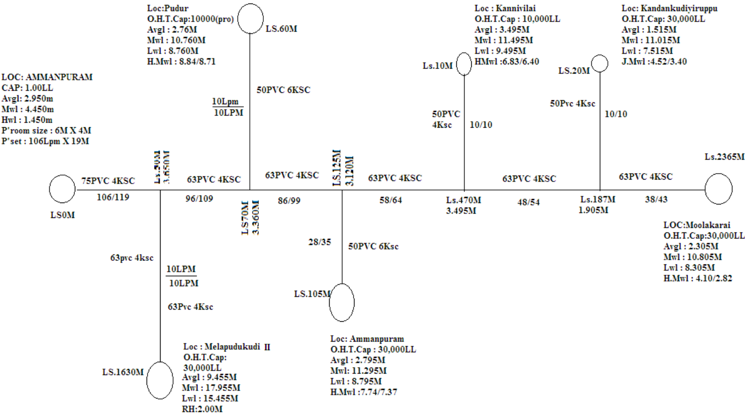
CWSS TO 159 RURAL HABITATIONS IN ALWARTHIRUNAGARI, THIRUCHENDUR, AND UDANGUDI UNIONS IN THOOTHUKUDI DISTRICT BRANCH MAIN FROM AMMANPURAM SUMP
