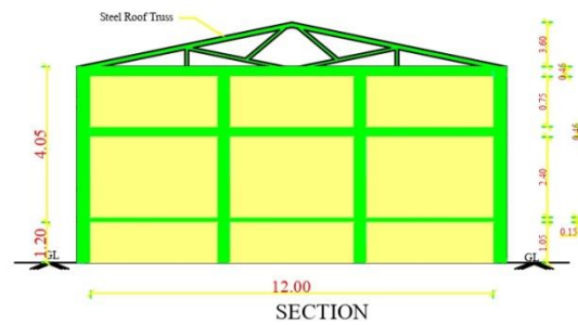
1000MT STORAGE GODOWN ELEVATION
