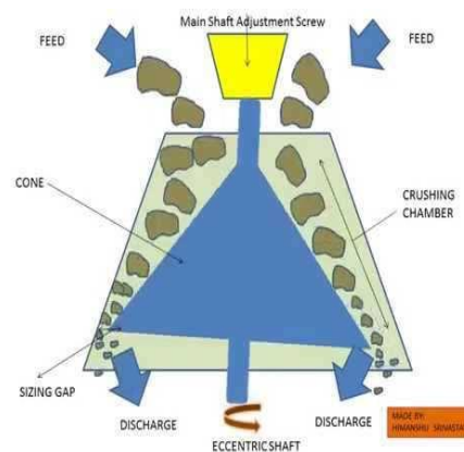
Cone Crusher
