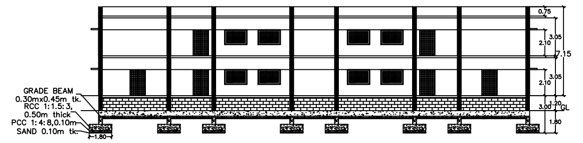
SECTION ON A-A
