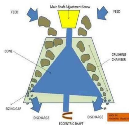
Cone Crusher
