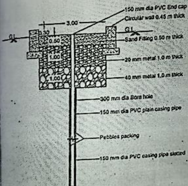
Typical Cross Section of Recharge Shaft
