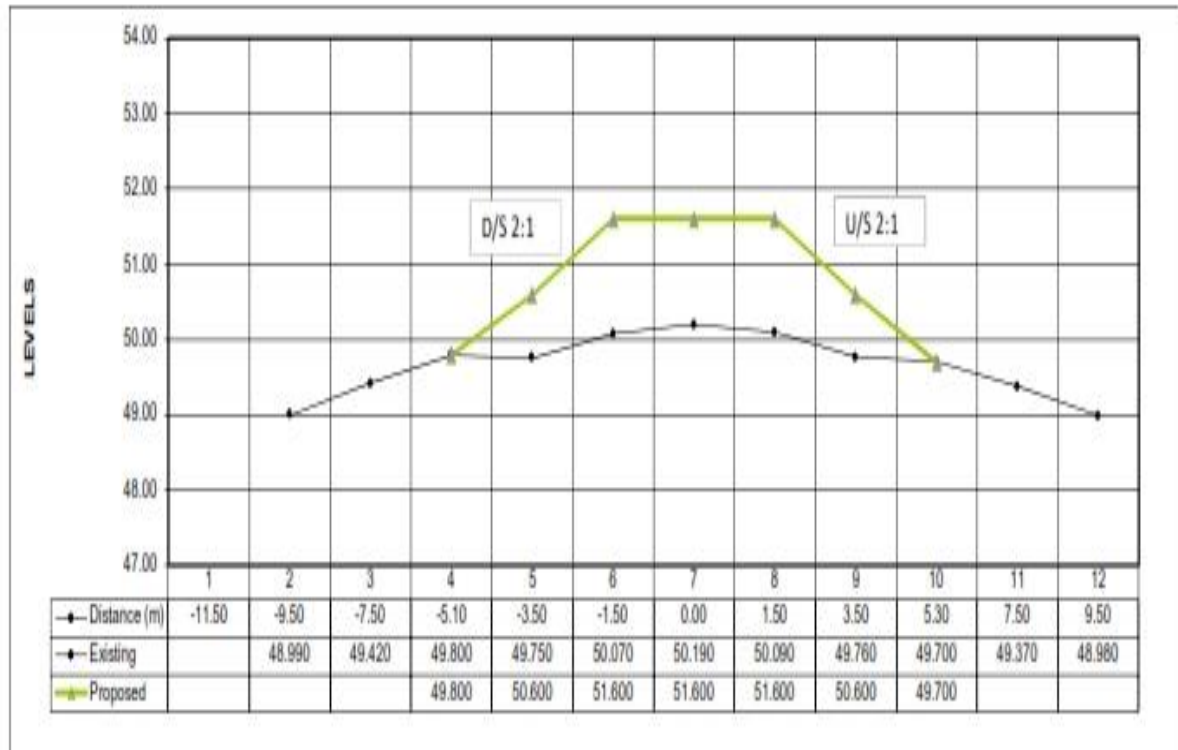
TYPICAL CROSS SECTION FOR TANK BUND
