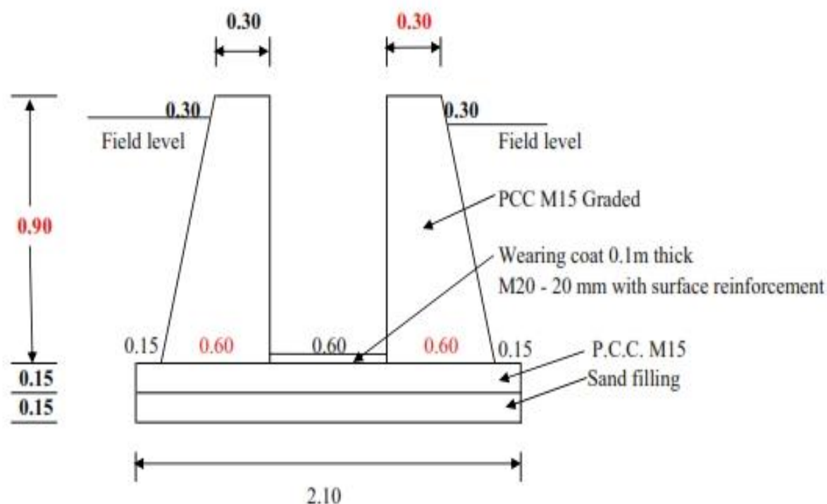
TYPICAL SECTION FOR FIELD CHANNEL
