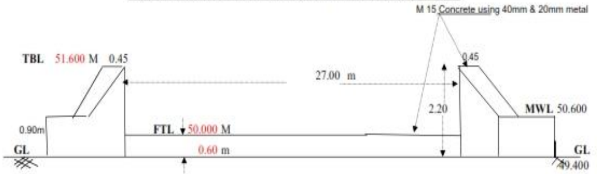
HALF SECTIONAL PLAN
