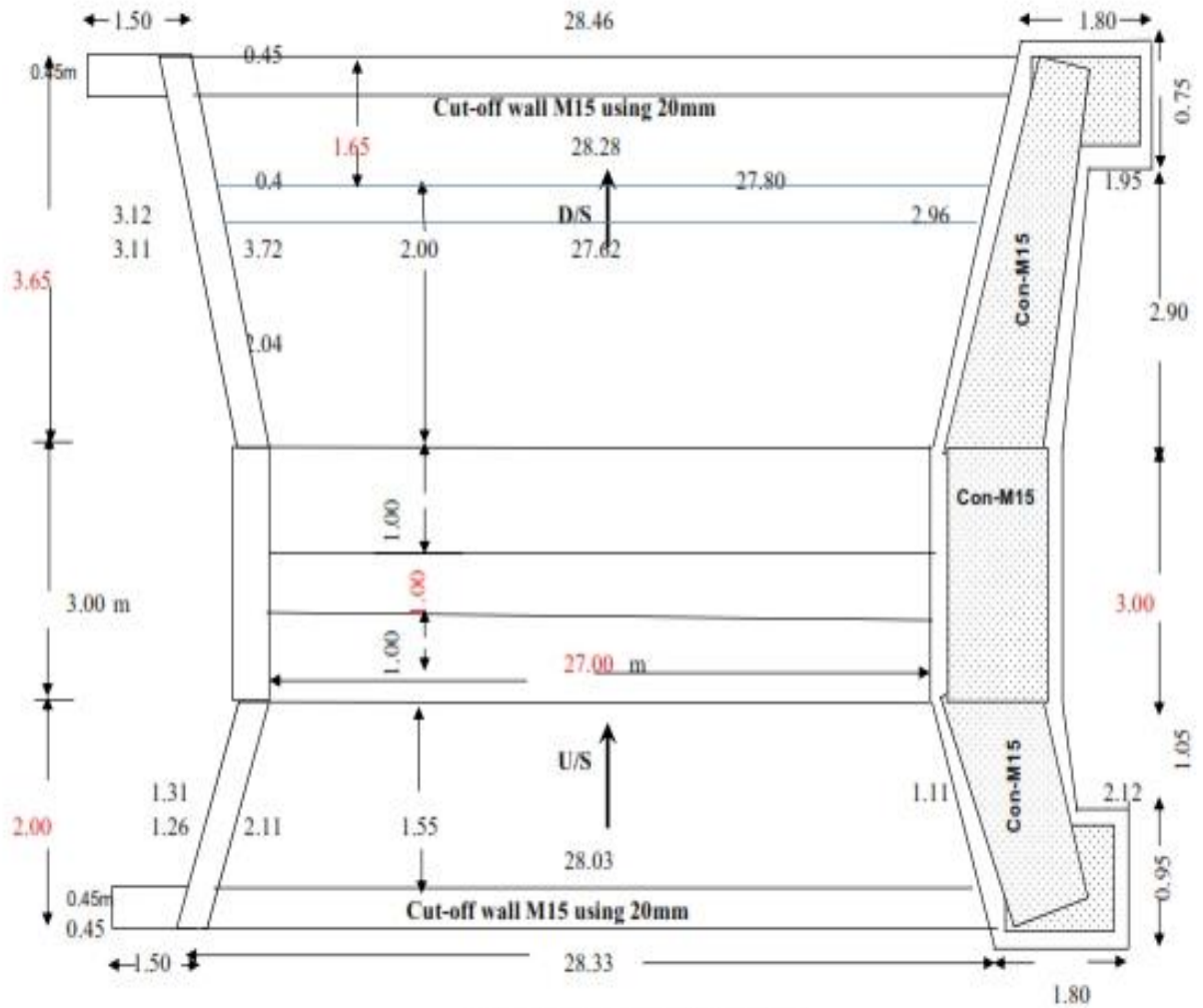
HALF SECTIONAL PLAN
