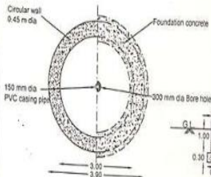
Typical Plan of Recharge Shaft
