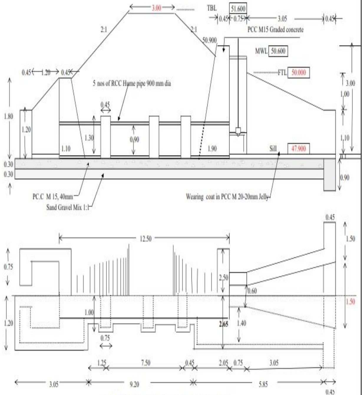
HALF PLAN AT TOP AND HALF PLAN AT BOTTOM
