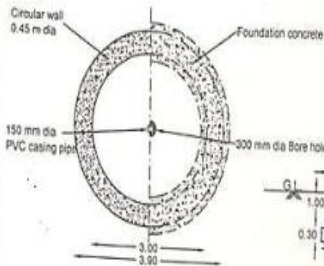
Typical Plan of Recharge Shaft
