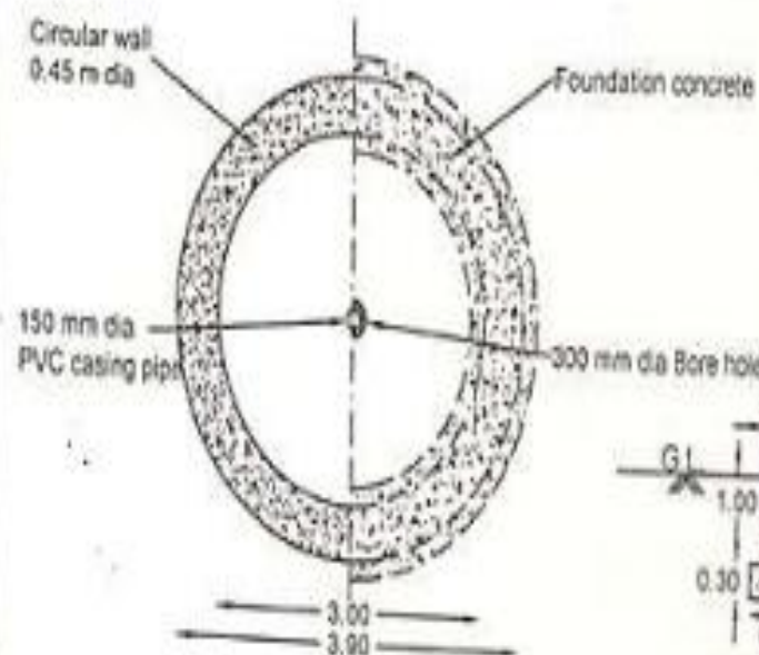
Typical Plan of Recharge Shaft
