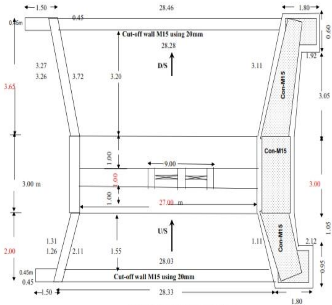
HALF SECTIONAL PLAN
