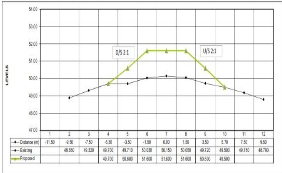
TYPICAL CROSS SECTION FOR TANK BUND
