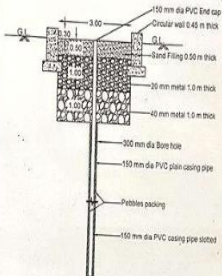
Typical Cross Section of Recharge Shaft
