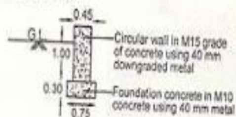
Details of Circular Wall
