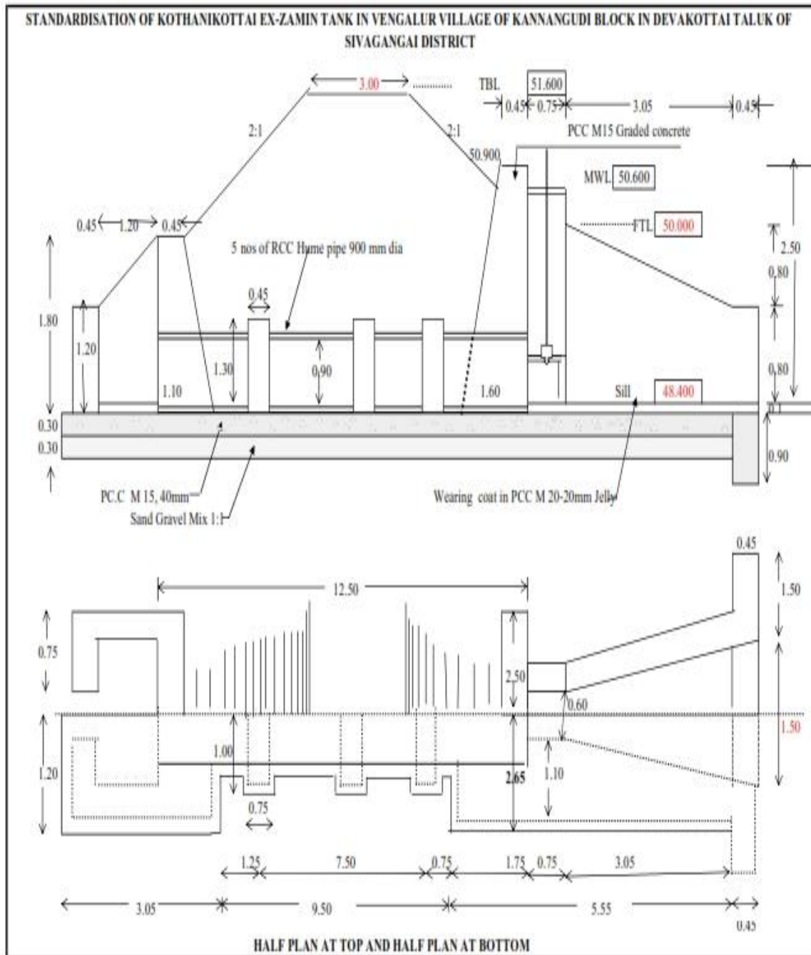
TYPICAL SECTION FOR SLUICE
