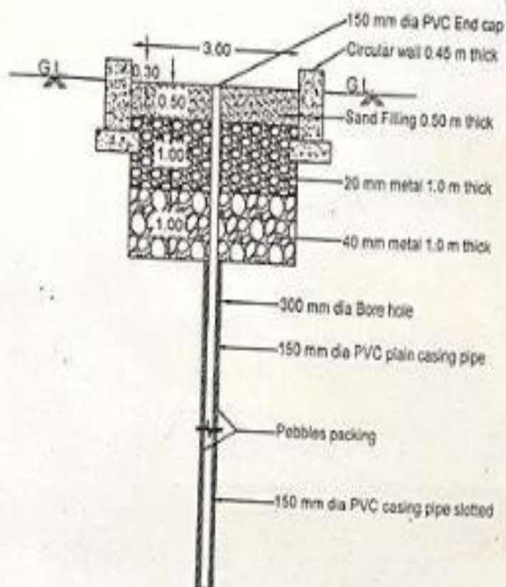
Typical Cross Section of Recharge Shaft
