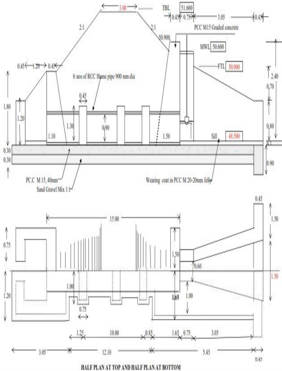
TYPICAL SECTION FOR SLUICE
