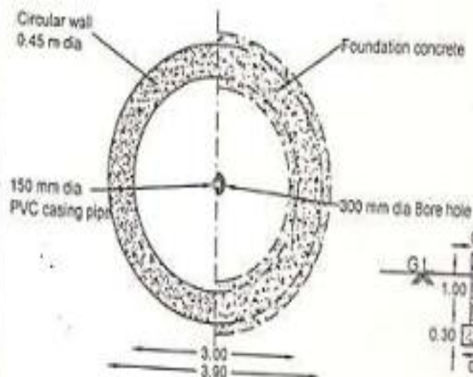
Typical Plan of Recharge Shaft
