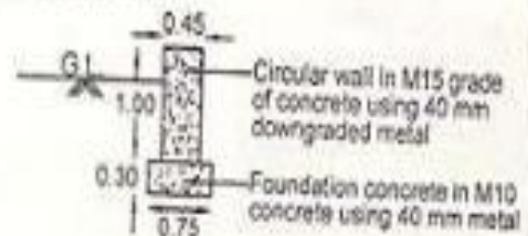
Details of Circular Wall
