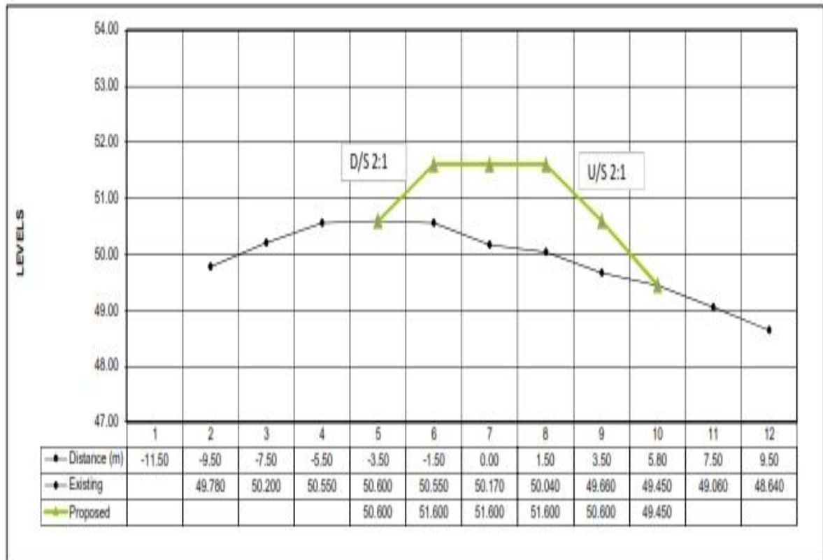
TYPICAL CROSS SECTION FOR TANK BUND
