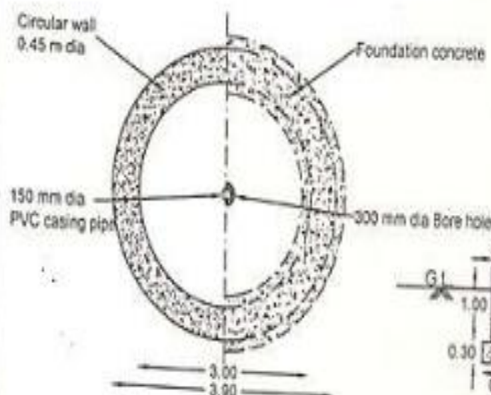
Typical Plan of Recharge Shaft
