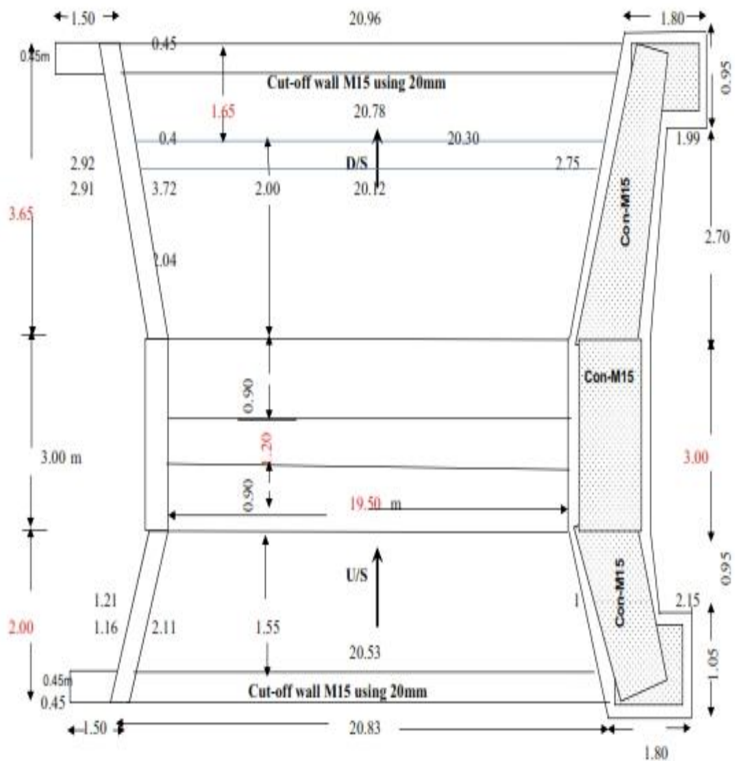
HALF SECTIONAL PLAN
