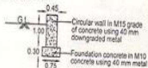
Details of Circular Wall
