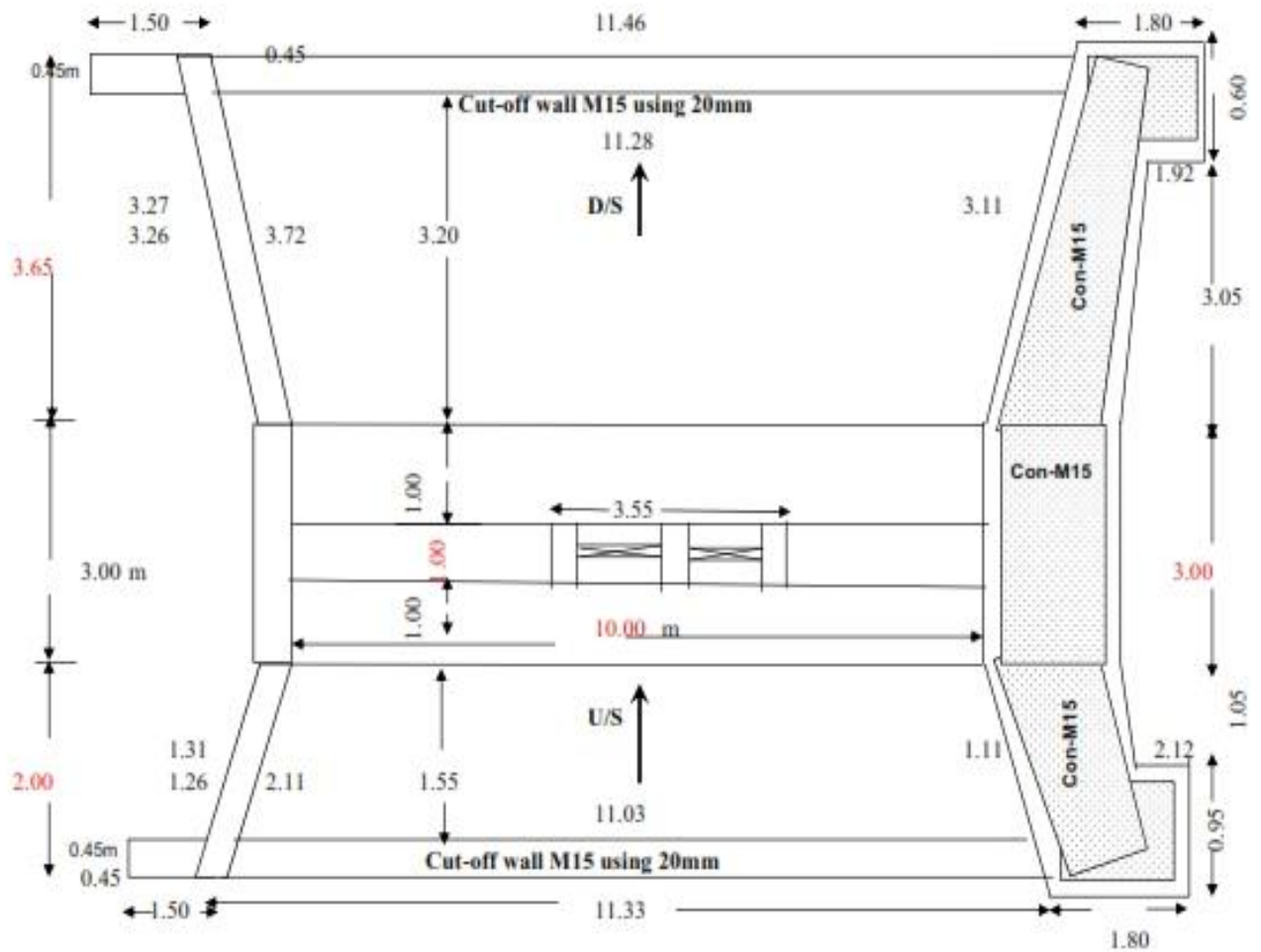
HALF SECTIONAL PLAN
