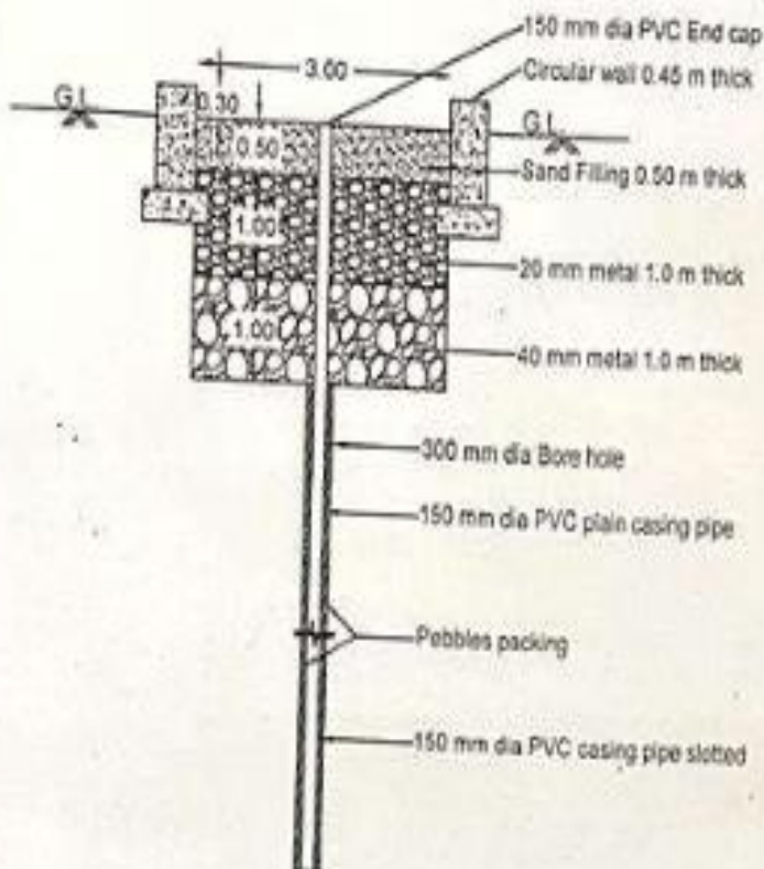
Typical Cross Section of Recharge Shaft
