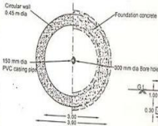
Typical Plan of Recharge Shaft
