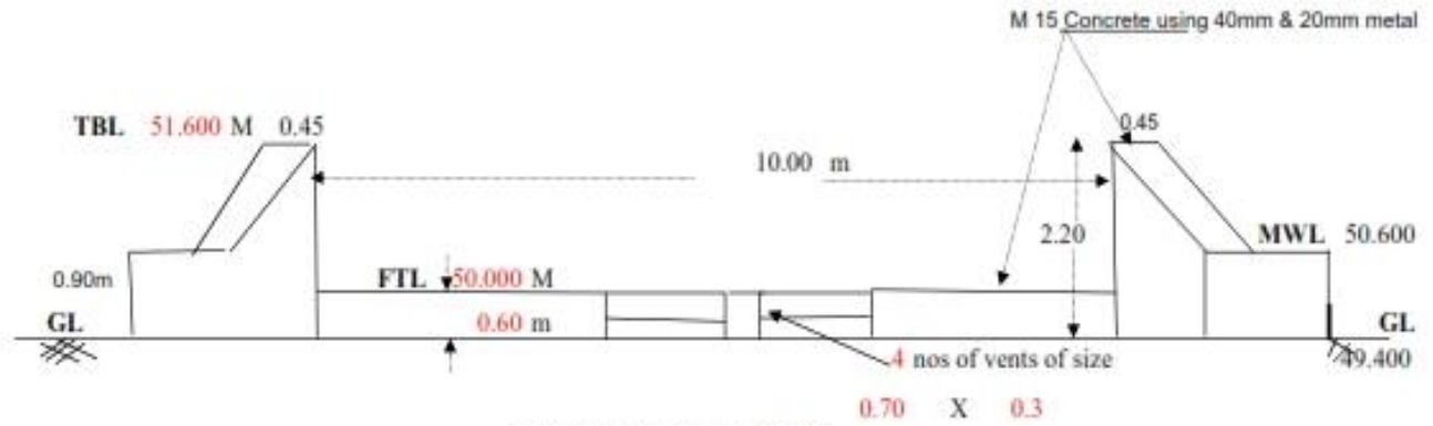
HALF SECTIONAL PLAN
