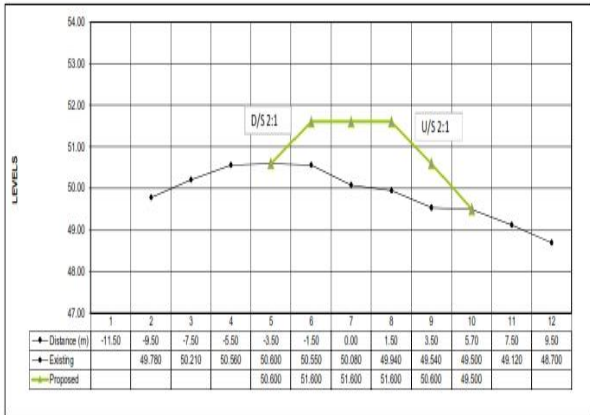
TYPICAL CROSS SECTION FOR TANK BUND
